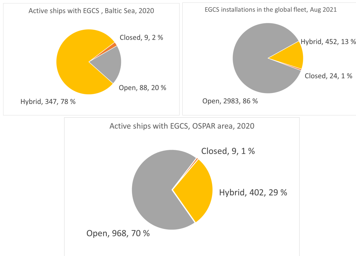
Figure 18. EGCS installations by equipment type, global fleet. Based on data collected from IMO GISIS on Aug 8th 2021.
