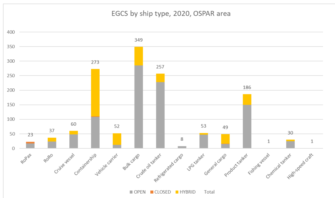
Figure 16. Installation of EGCS by ship type in the OSPAR Region. This allocation is based on vessels which were active during 2020 in the OSPAR domain.
