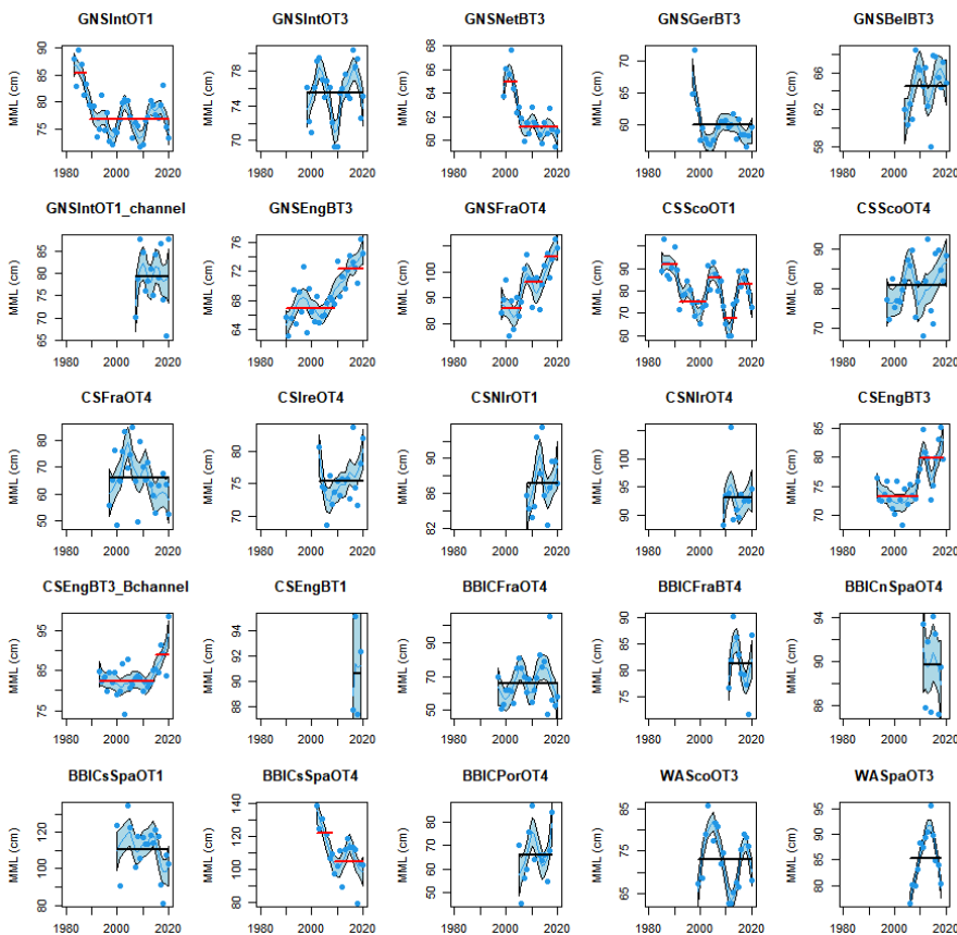
Figure 2: Time series of mean maximum length by survey showing data points, LOESS smoothed patterns and stable periods (black if constant over period assessed and red if a breakpoint is detected).
