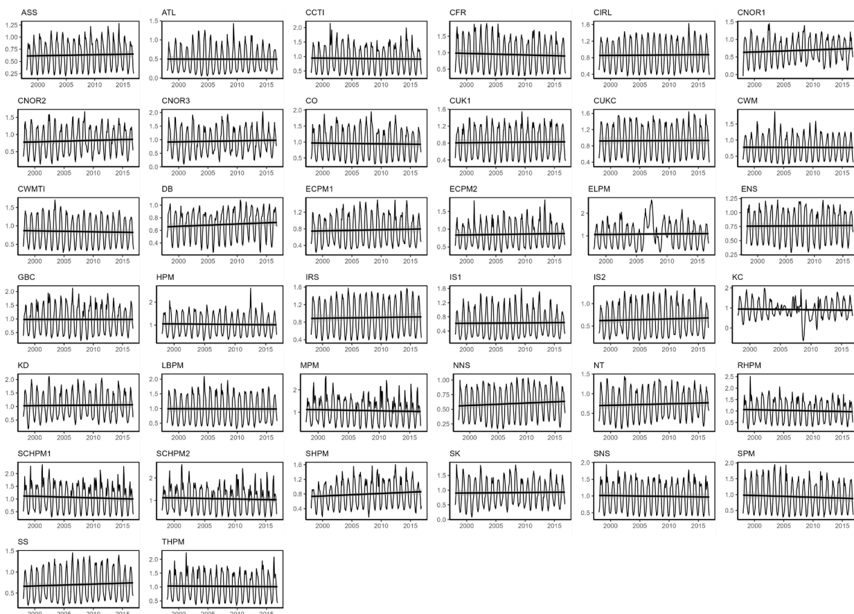
Figure b: Time-series (1997-2016) of primary production and their trends within each assessment unit.
