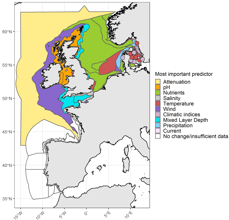
Figure 3: Most important variables addressing changes in primary production within the COMP4 assessment units.
