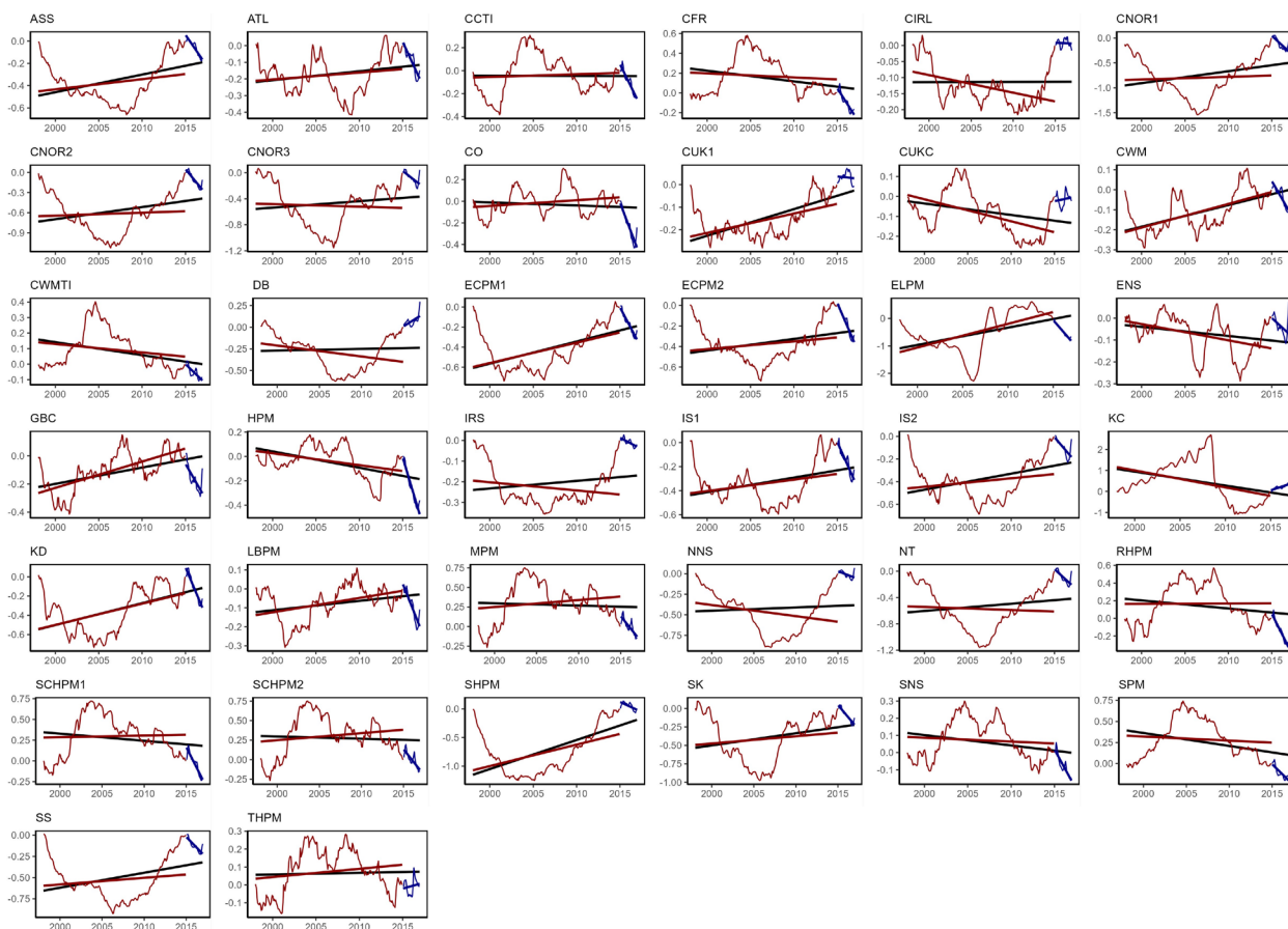
Figure c: Cumulative sum of the primary production monthly anomalies. The line in red represents the anomalies of the reference period. The line in blue represents the anomalies of the assessment period.
