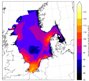
Figure 3: Median total Sound Pressure Level, 125 Hz band. Below monthly maps for January (left) and July (right) 2019.
