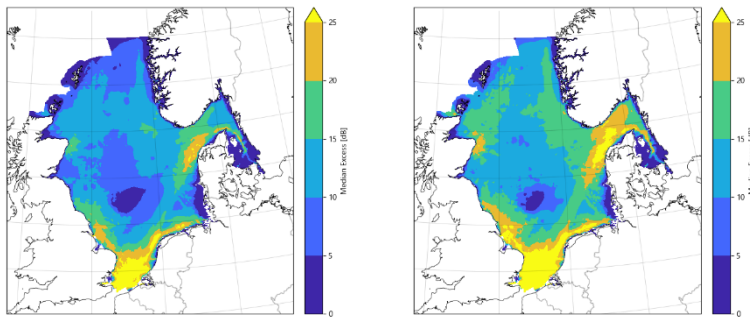
Figure 4: Median Excess Level, 125 Hz band. Below monthly maps for January (left) and July (right) 2019.
