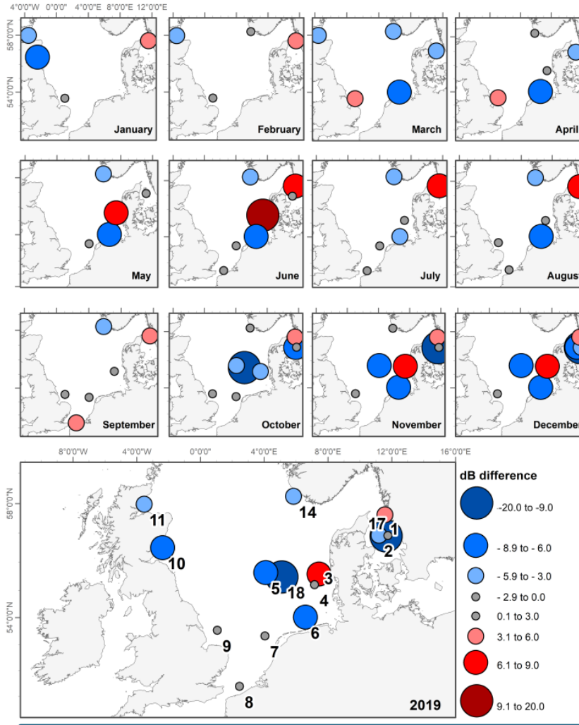
Map: Difference between passive acoustic monitoring and modelled decibel levels for the JOMOPANS stations between 20 - 20000 Hz. (Positive value indicates the model is overestimating the PAM data and negative value indicates the model is underestimating the PAM data.) Top 12 plots show the monthly P50 value for each station and bottom plot shows the yearly P50 value.
