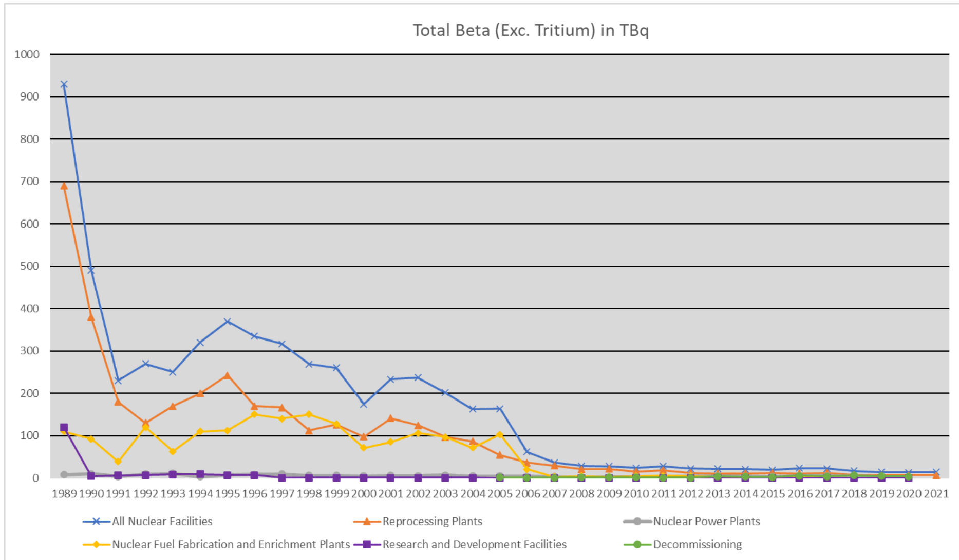
Figure 3. Total beta discharges 1989 – 2021 (in TBq) – Achievements of the OSPAR Convention signed in 1992
