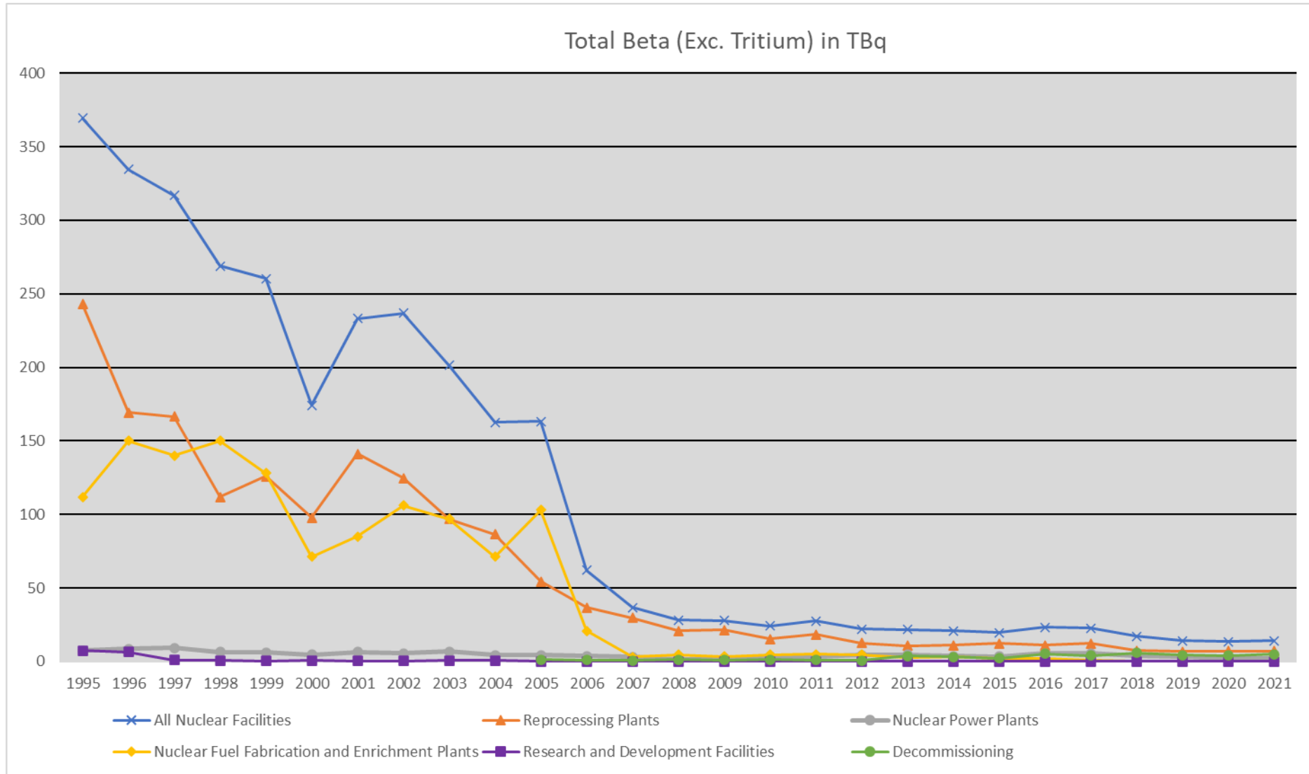
Figure 6. Total beta discharges 1995 – 2021 (in TBq) – Achievements of the OSPAR Strategy adopted in Sintra in 1998
