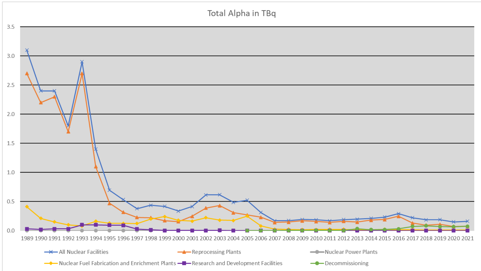
Figure 1. Total alpha activity discharges 1989 – 2021 (in TBq) – Achievements of the OSPAR Convention signed in 1992
