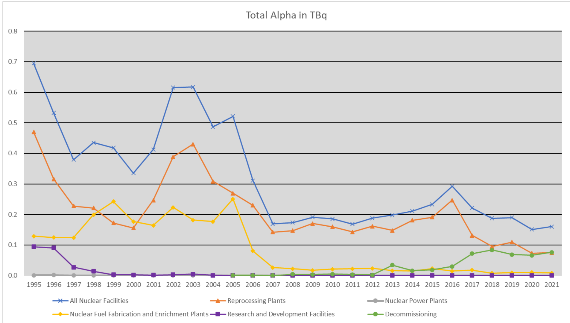
Figure 4. Total alpha activity discharges 1995 – 2021 (in TBq) – Achievements of the OSPAR Strategy adopted in Sintra in 1998
