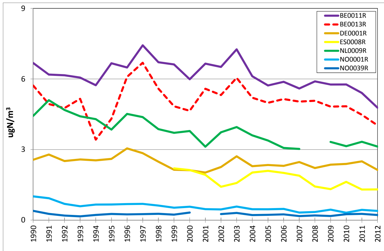
Figure 4.1: Time series of \text{NO}_2 . Time series of solid lines are sites with significant trends while dotted lines are not.
