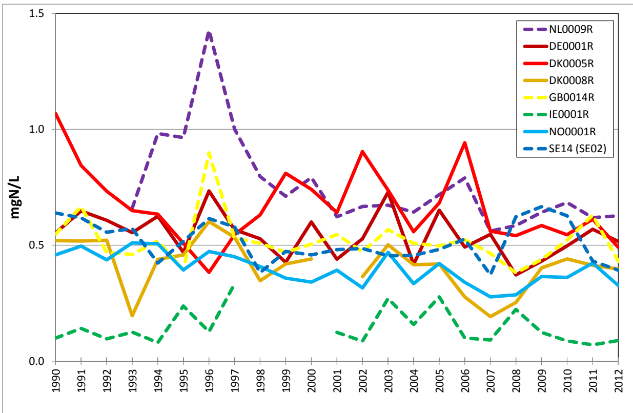
Figure 4.5: Time series of \text{NH}_4 in precipitation. Solid lines are sites with significant trends while dotted lines are not.
