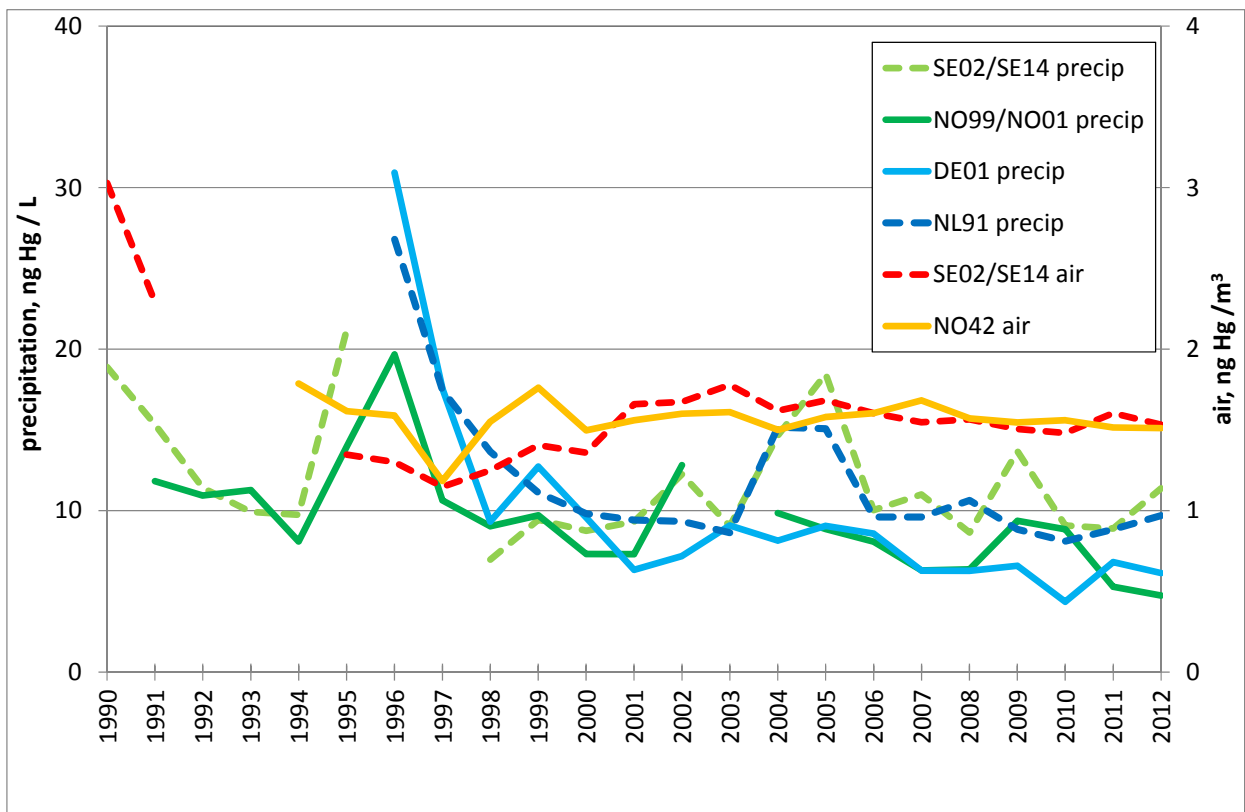
Figure 4.10: Time series of mercury. Solid lines are sites with significant trends while dotted lines are not.
