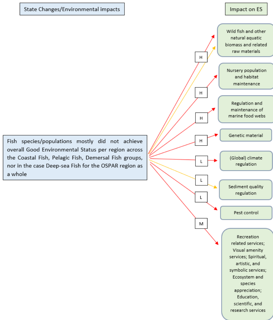
Figure I.1: Schematic depicting the 'State (changes)' - 'Impacts on ES' linkages for the Fish Thematic Assessment. The ecosystem services shown are those considered most relevant to the Fish Thematic Assessment. Each arrow also denotes an expert estimate of the nature and magnitude of the impact (yellow arrow = neutral impact, red arrow = negative impact; H = high impact, M = medium impact, L = low impact)
