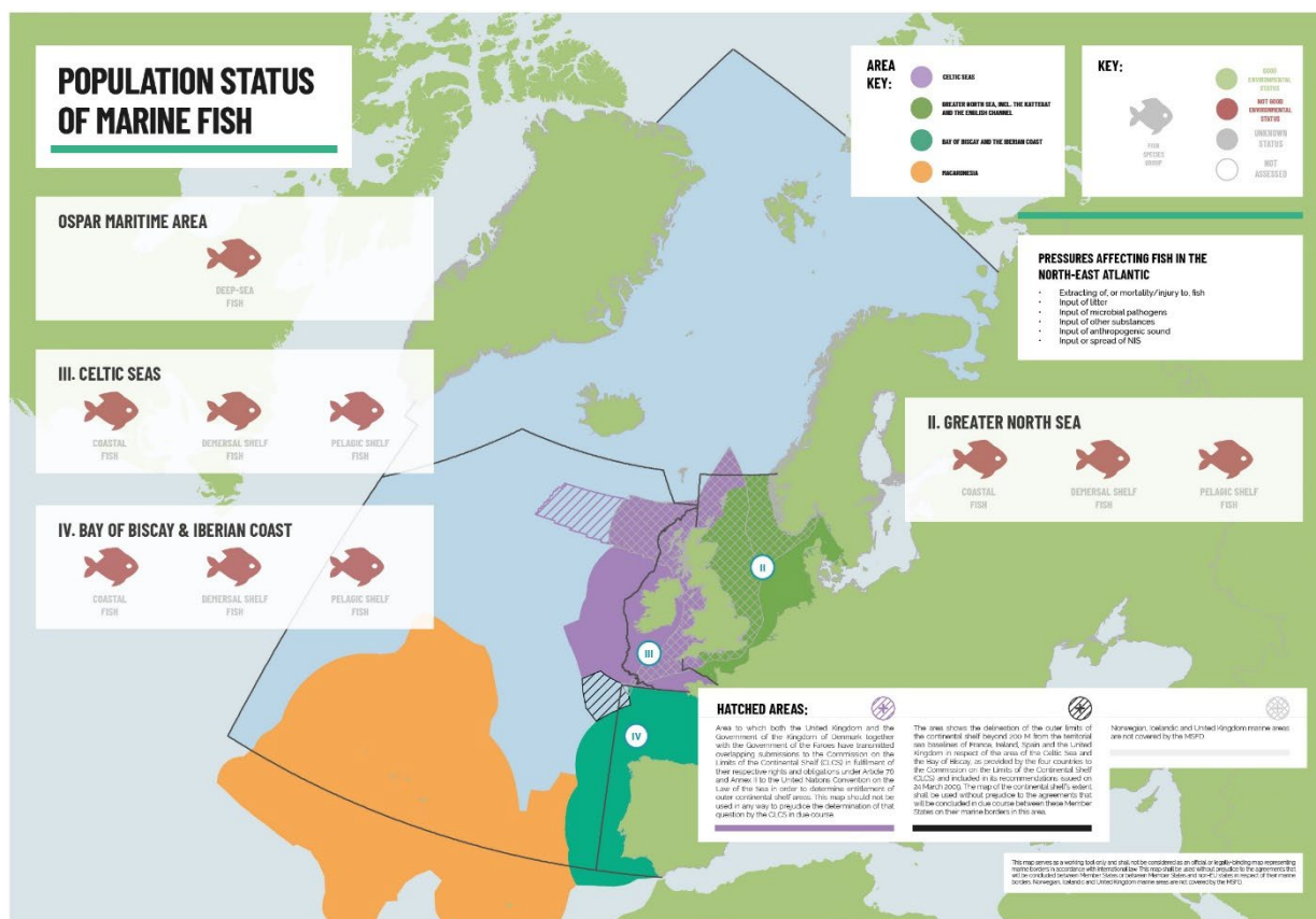
Figure S.1: Schematic representation of good environmental status of fish by species group and spatial assessment unit, based on the integrated fish assessment. Norwegian, Icelandic and United Kingdom marine areas are not covered by the MSFD.
