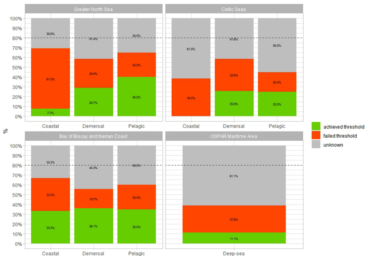
Figure S.2: Proportion of fish having achieved or failed the threshold for each species group and spatial assessment unit. To achieve good environmental status for the integrated status assessment of fish species groups, 80% of the items per group must have achieved their threshold. Assessment reference period 2015-2020.
