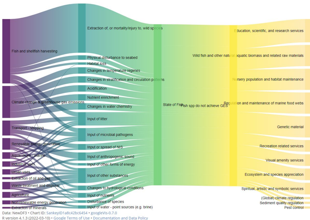
Figure CE.1: Impact Potential of Fish to exposure to pressures from human activities in the North-East Atlantic. Columns left to right: Activity, Pressure, State, Environmental Impact, Ecosystem Service. Derived from Exposure score (Extent x Frequency of pressure) x Degree of Impact score (in terms of whether impact is Acute or Chronic). Pressures with a low Degree of Impact score have been removed for clarity. ‘Impact’ in this context does not consider the persistence of the pressure or the resilience of the ecosystem associated with that pressure. Were these parameters to be included, the relative contribution for some pressures would most likely increase and score higher in the relative ranking. Links are weighted to indicate relative contribution to impact. A wider link = greater potential for impact
