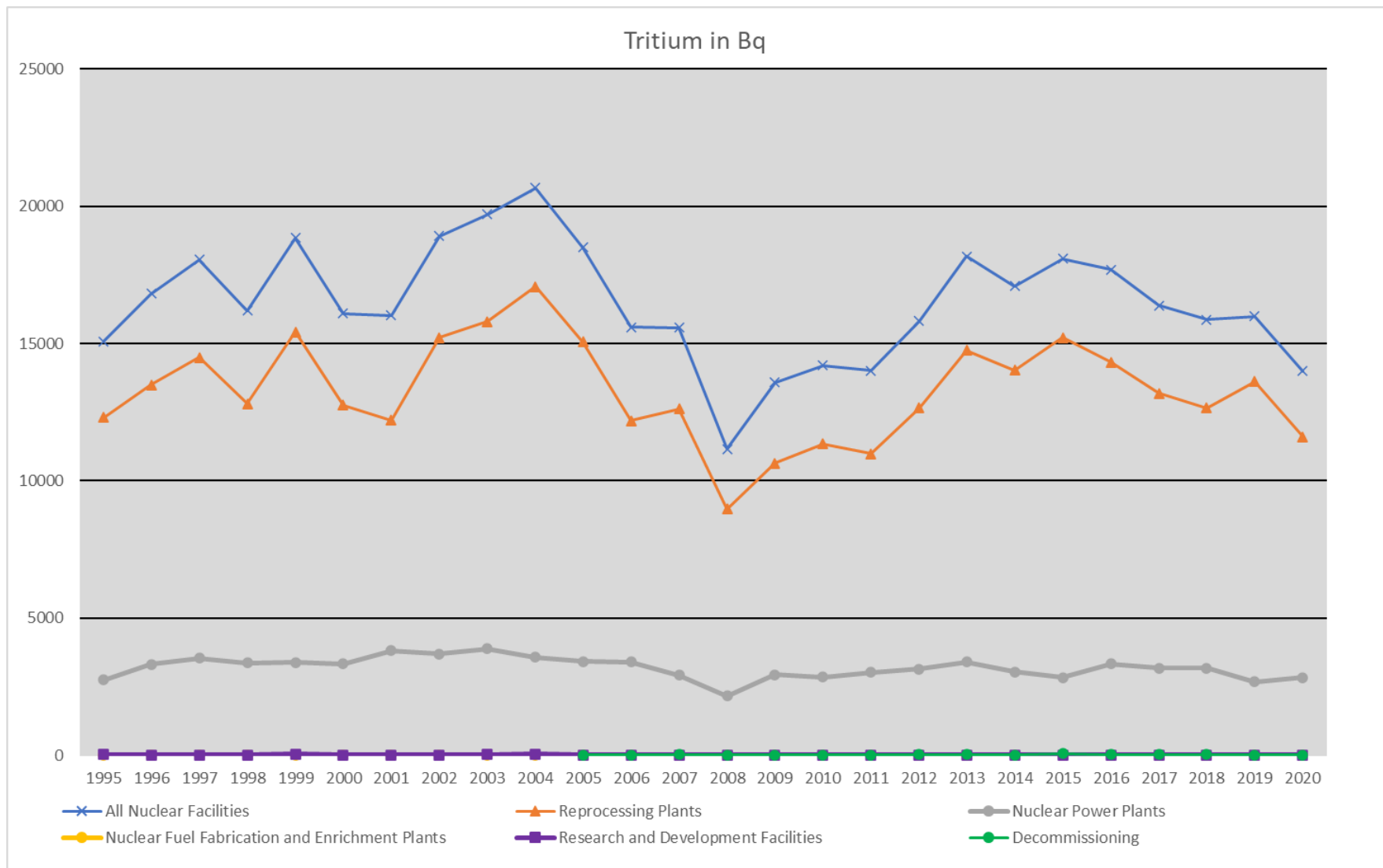
Figure 5. Discharges of tritium 1995 – 2019 (in TBq) – Achievements of the OSPAR Strategy adopted in Sintra in 1998
