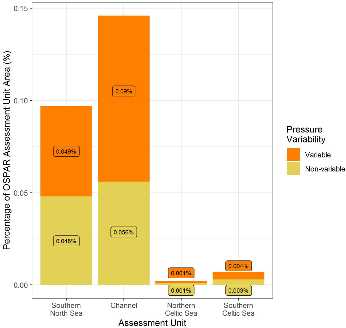
Figure ak33: Percentage of OSPAR Common Indicator Assessment Unit with 'Non-variable' or 'Variable' pressure in the 2009 to 2020 assessment period; cells were categorised 'Variable' if a range of three or more pressure categories was observed throughout the time series.
