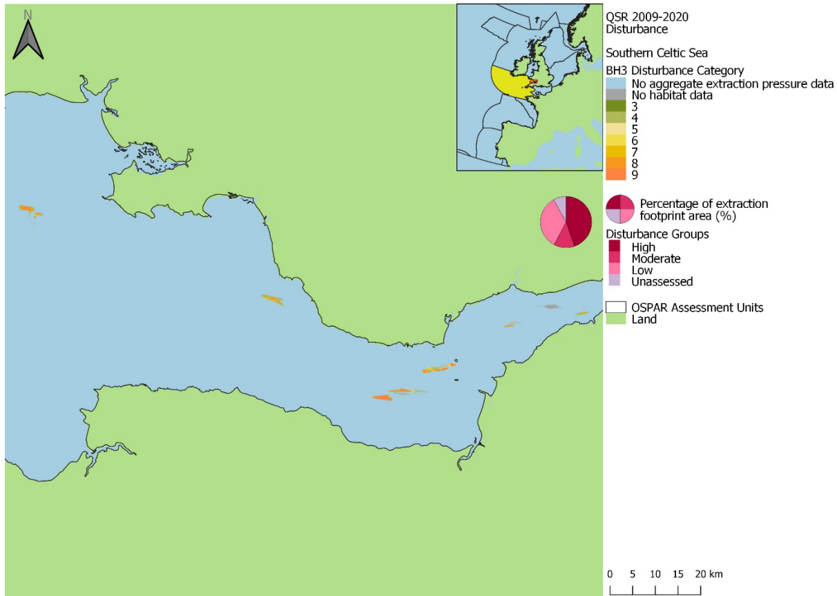
Figure bm61: Spatial distribution of extraction disturbance within the Southern Celtic Sea assessment unit in the 2009 to 2020 assessment period. Pie charts show the percentage of the extraction footprint area under each disturbance group: 'High' (categories 8-9), 'Moderate' (categories 5-7), 'Low' (categories 1-4), and Unassessed (area where extraction pressure was present, but disturbance could not be assessed due to i) no habitat data, or ii) no sensitivity assessments for underlying habitat).
