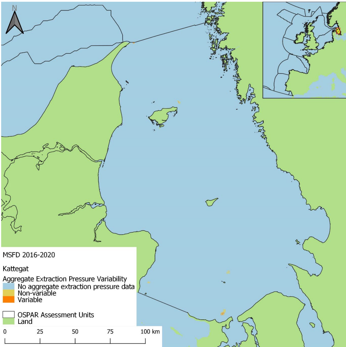
Figure ay47: Spatial distribution of 'Variable' and 'Non-variable' extraction pressure in the 2016 to 2020 assessment period in the Kattegat assessment unit. Grid cells were categorised 'Variable' if a range of three or more pressure categories was observed throughout the time series.
