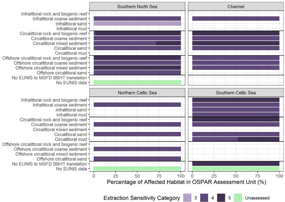
Figure w19: Percentage of sensitivity categories for Broad Habitat Types in OSPAR Common Indicator Assessment Units with extraction pressure in the 2009 to 2020 assessment period.
