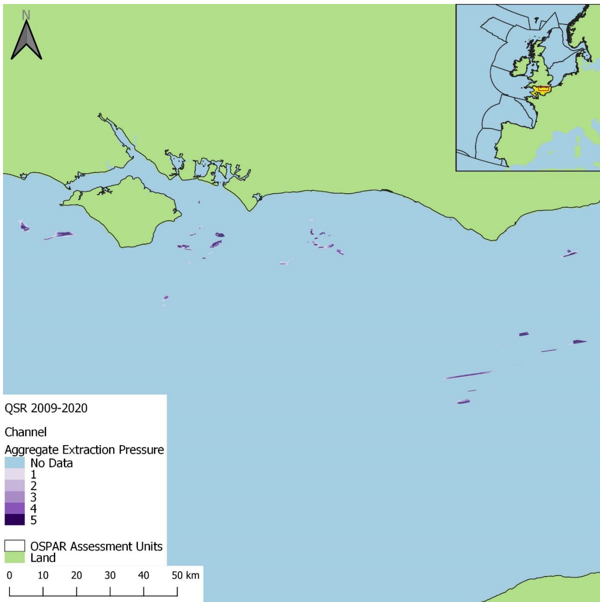
Figure aa23: Aggregated extraction pressure in the 2009 to 2020 assessment period, within the Channel assessment unit.
