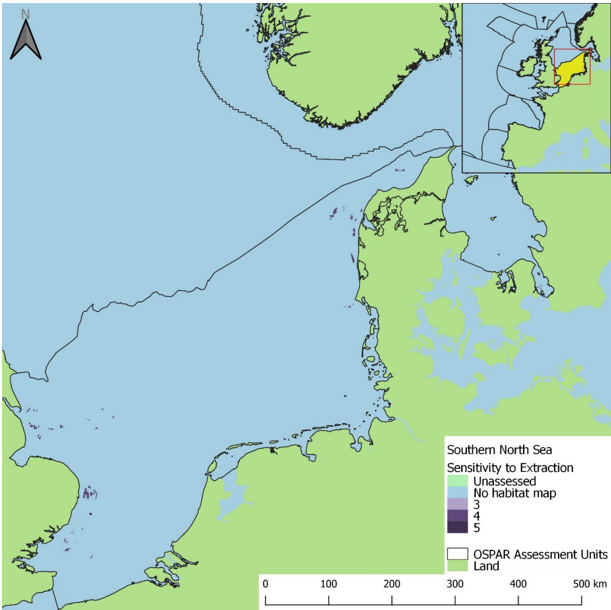
Figure p12: Extent and distribution of habitat and benthic species sensitivities (based on resilience and resistance) to extraction combined within EUNIS Level 2-6 benthic habitat types, where aggregate extraction pressure data were available in the Southern North Sea assessment unit.
