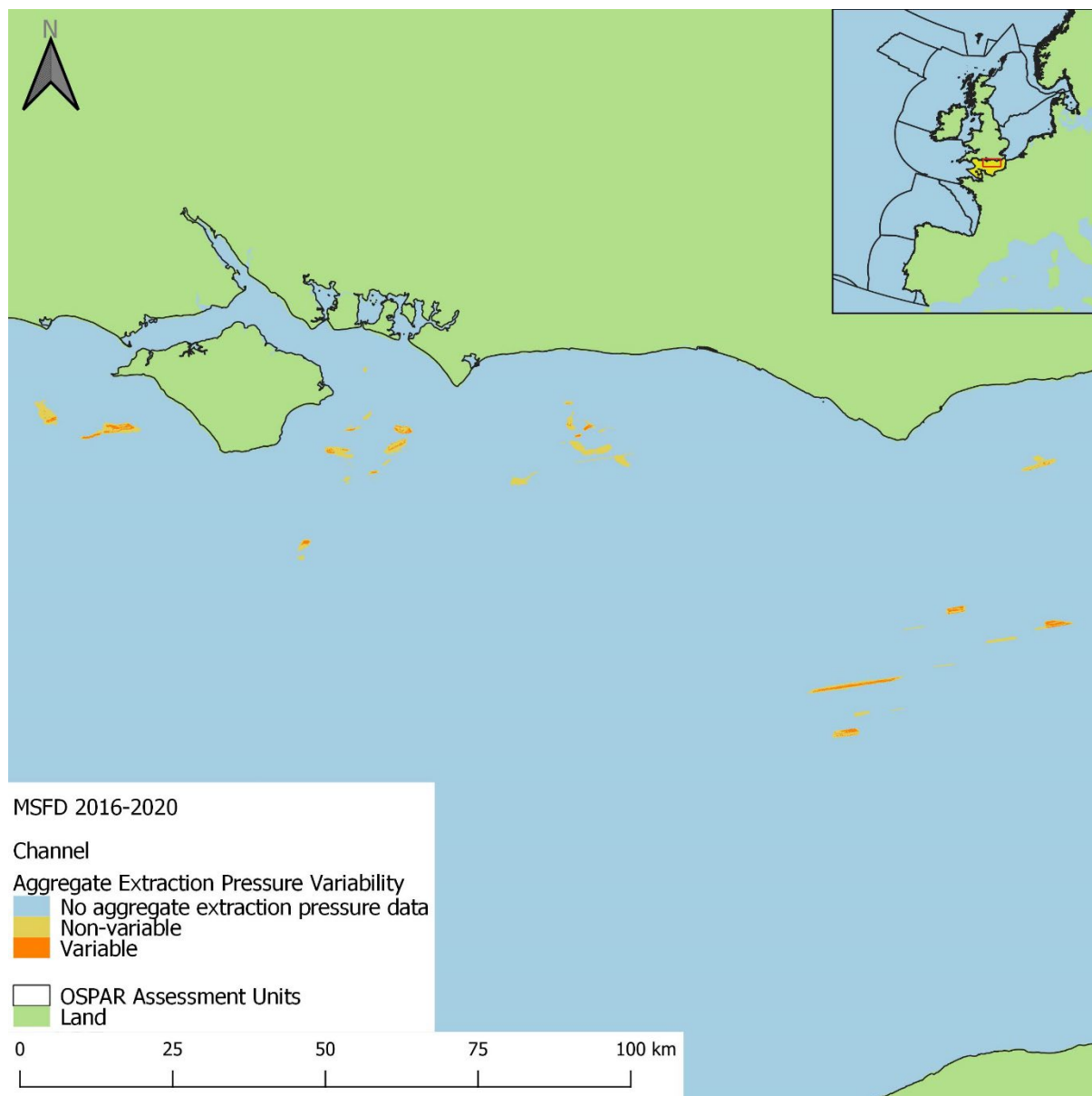
Figure aw45: Spatial distribution of 'Variable' and 'Non-variable' extraction pressure in the 2016 to 2020 assessment period in the Channel assessment unit. Grid cells were categorised 'Variable' if a range of three or more pressure categories was observed throughout the time series.
