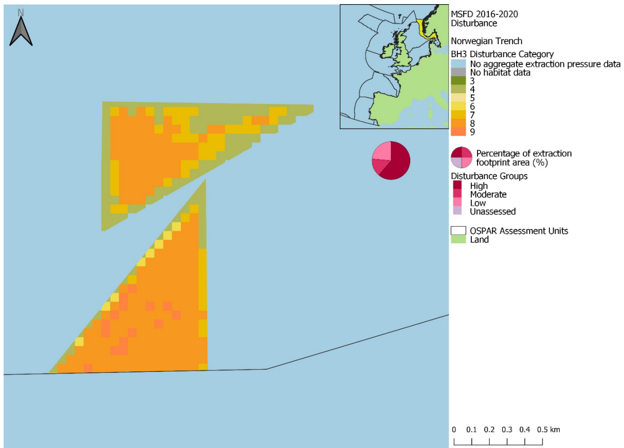
Figure bu69: Spatial distribution of extraction disturbance within the Norwegian Trench assessment unit in the 2016 to 2020 assessment period. Pie charts show the percentage of the extraction footprint area under each disturbance group: ‘High’ (categories 8-9), ‘Moderate’ (categories 5-7), ‘Low’ (categories 1-4), and Unassessed (area where extraction pressure was present, but disturbance could not be assessed due to i) no habitat data, or ii) no sensitivity assessments for underlying habitat).
