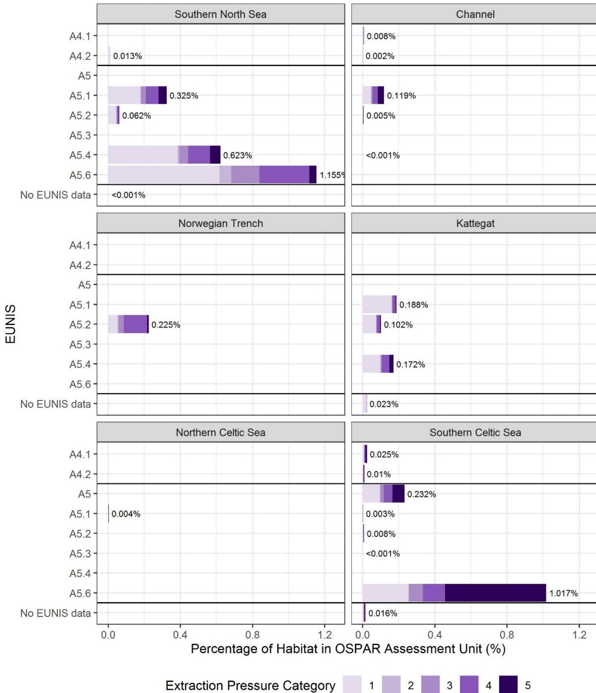
Habitats with Extraction Pressure in Common Indicator Assessment Units 2016 to 2020
