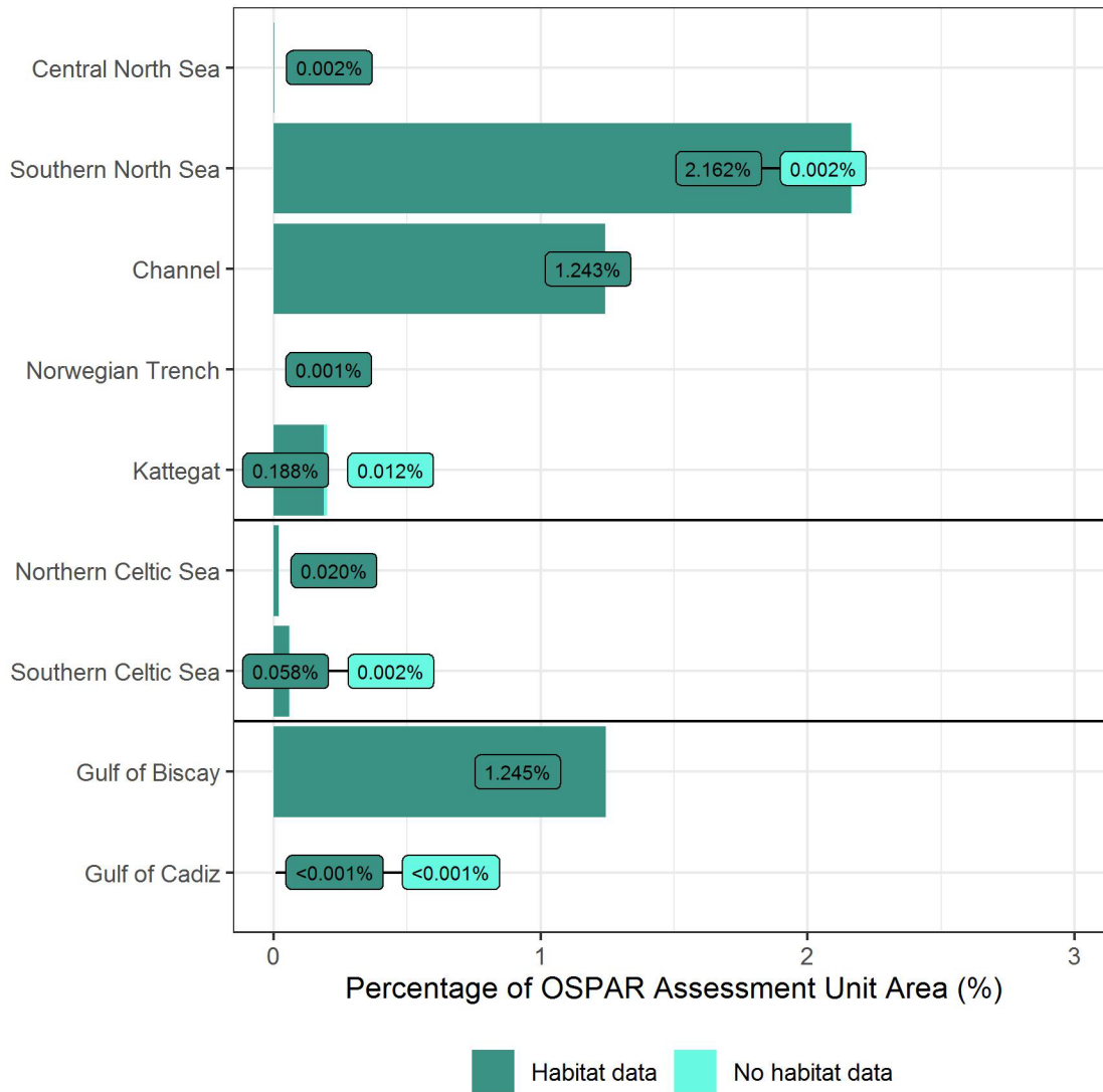
Figure n10: Percentage of OSPAR Common Indicator assessment units designated as licensed extraction areas; No habitat data = area where EUNIS habitat data were not available (habitat information unavailable or incompatible with EUNIS classification).
