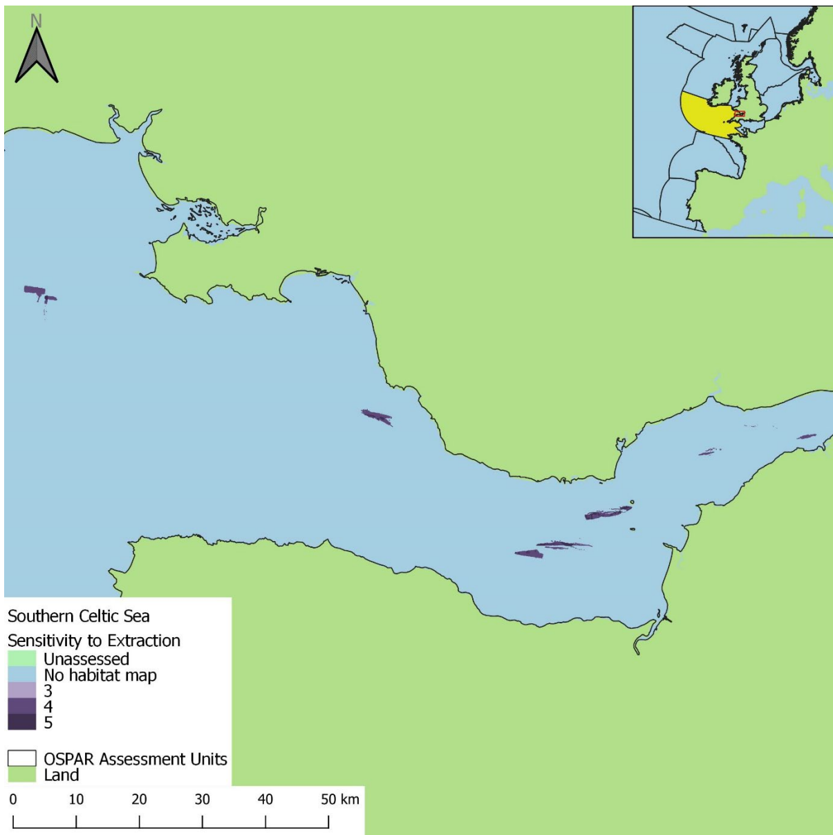
Figure u17: Extent and distribution of habitat and benthic species sensitivities (based on resilience and resistance) to extraction combined within EUNIS Level 2-6 benthic habitat types, where aggregate extraction pressure data were available in the Southern Celtic Sea assessment unit.
