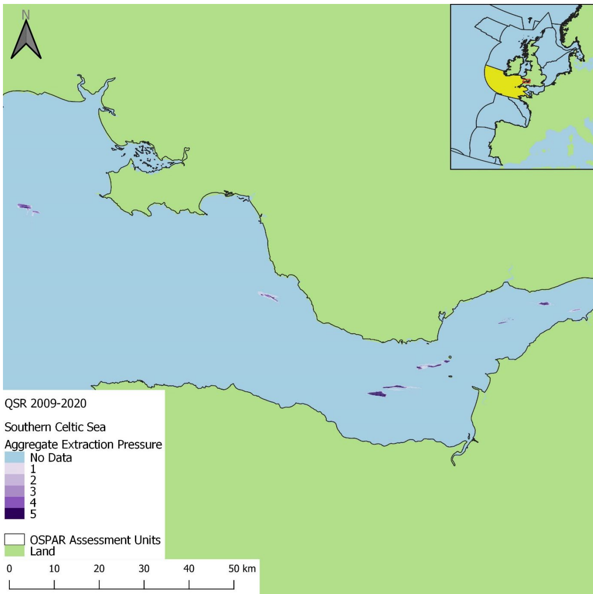
Figure ac25: Aggregated extraction pressure in the 2009 to 2020 assessment period, within the Southern Celtic Sea assessment unit.
