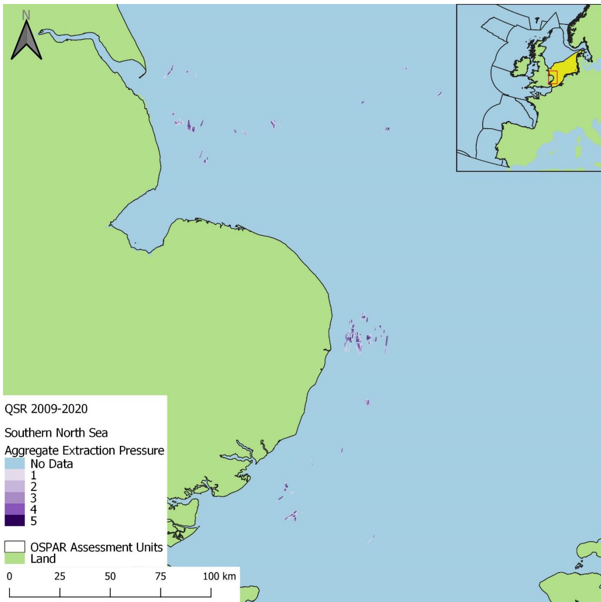
Figure z22: Aggregated extraction pressure in the 2009 to 2020 assessment period, within the Southern North Sea assessment unit.
