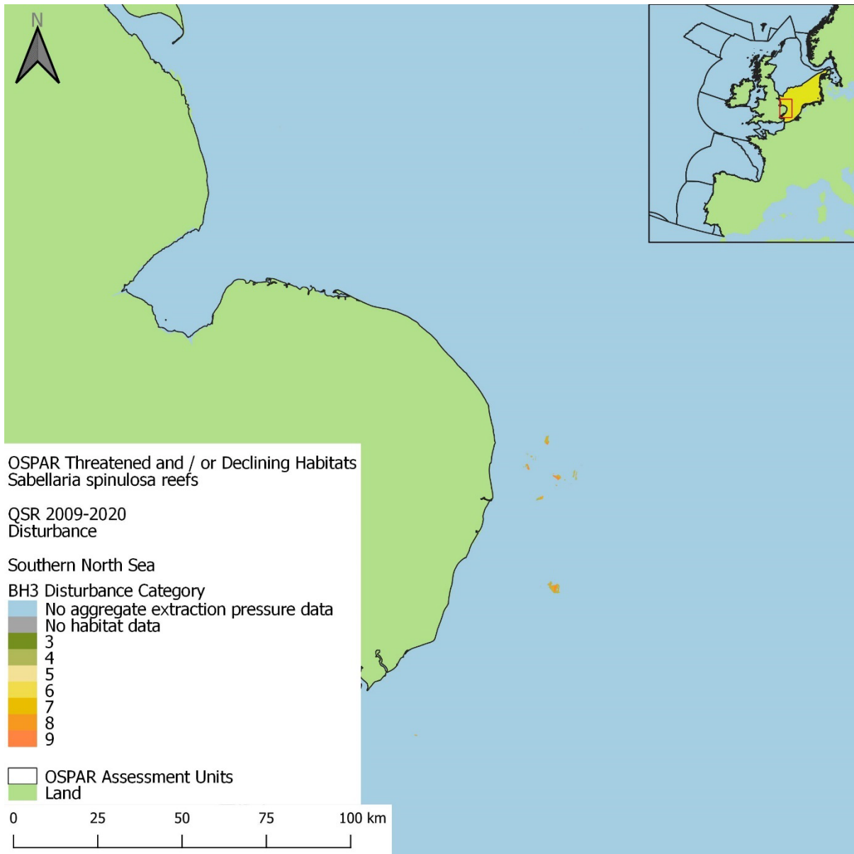
Figure ca75: Spatial distribution of aggregated disturbance for OSPAR Threatened and / or Declining Habitats ( Sabellaria spinulosa reefs) in the 2009 to 2020 assessment period.
