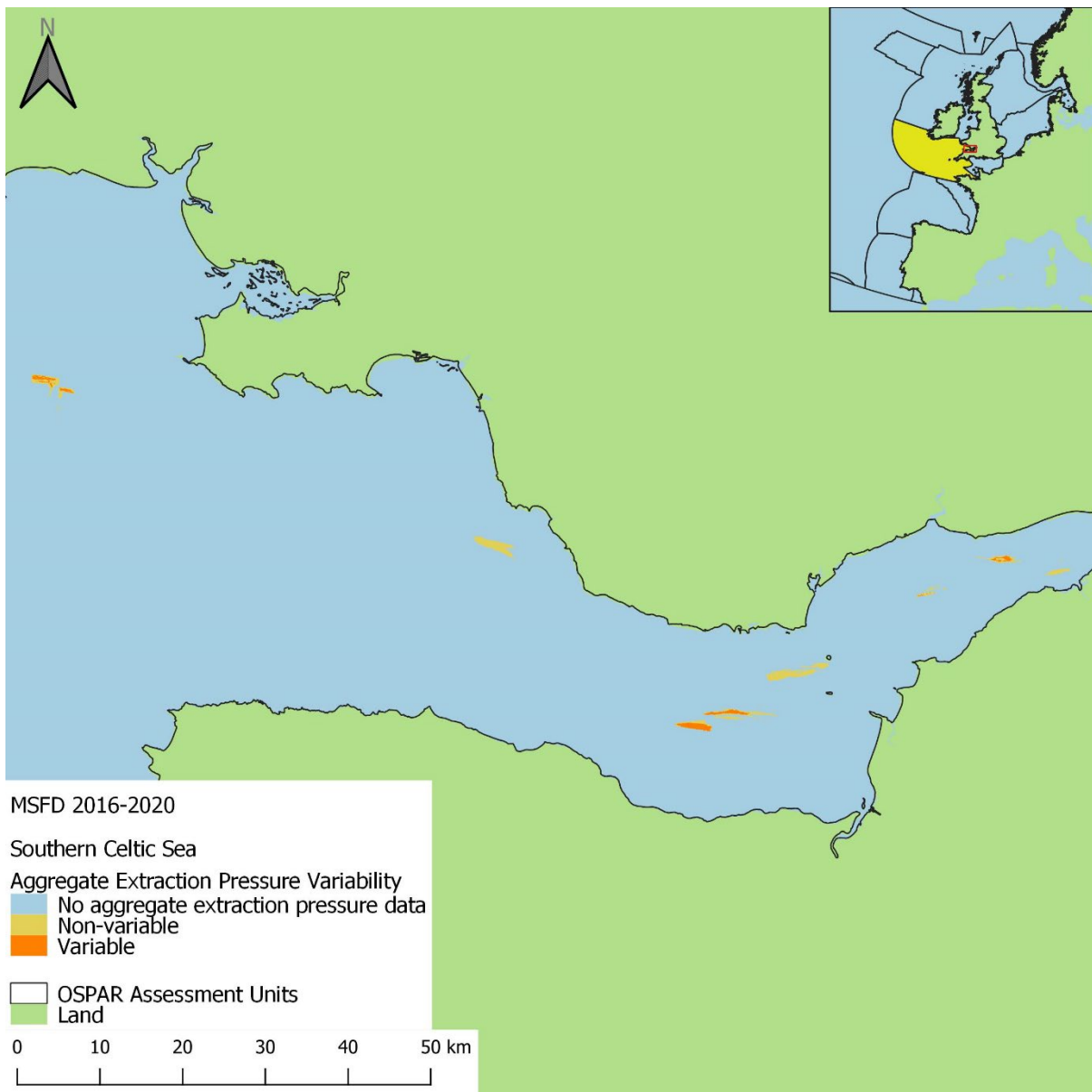
Figure ba49: Spatial distribution of 'Variable' and 'Non-variable' extraction pressure in the 2016 to 2020 assessment period in the Southern Celtic Sea assessment unit. Grid cells were categorised 'Variable' if a range of three or more pressure categories was observed throughout the time series.
