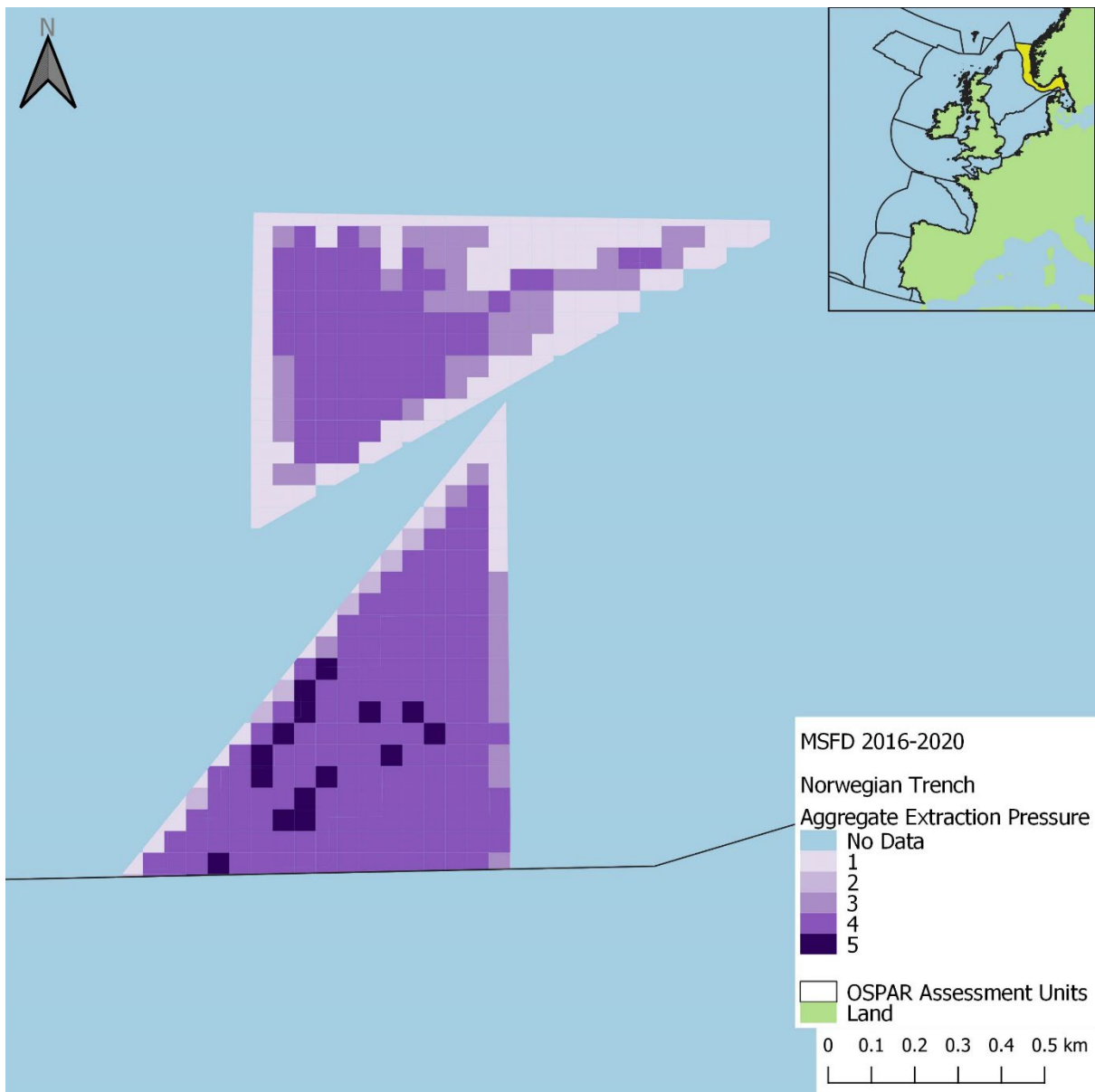
Figure ao37: Aggregated extraction pressure in the 2016 to 2020 assessment period, within the Norwegian Trench assessment unit.
