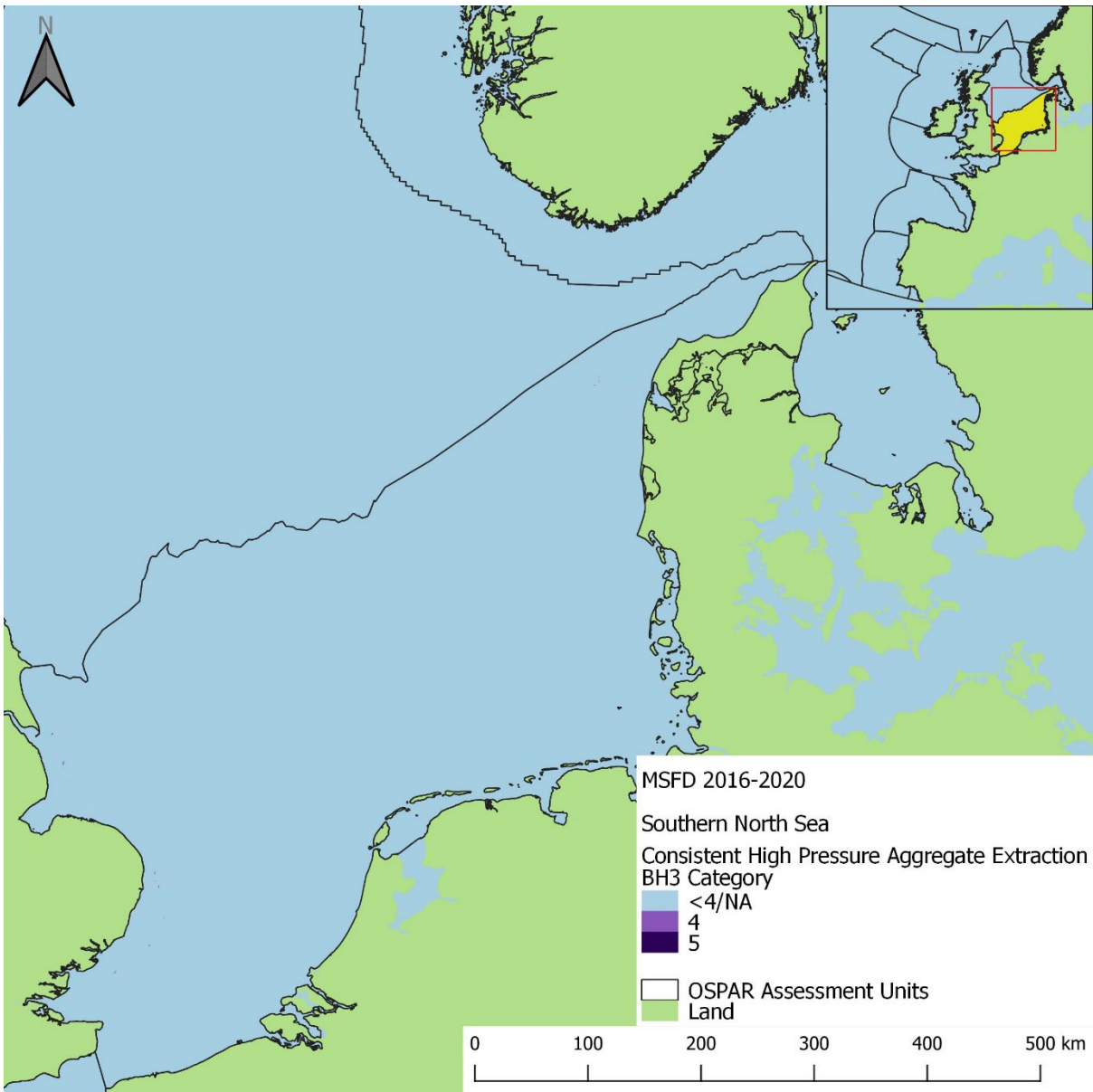
Figure bc51: Spatial distribution of consistently high (category 4 or 5) extraction pressure within the 2016 to 2020 assessment period in the Southern North Sea assessment period. Grid cells were considered to have 'Consistent' pressure if a change in less than three pressure categories was observed within the assessment period.
