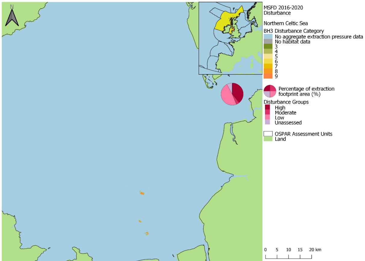
Figure bw71: Spatial distribution of extraction disturbance within the Northern Celtic Sea assessment unit in the 2016 to 2020 assessment period. Pie charts show the percentage of the extraction footprint area under each disturbance group: ‘High’ (categories 8-9), ‘Moderate’ (categories 5-7), ‘Low’ (categories 1-4), and Unassessed (area where extraction pressure was present, but disturbance could not be assessed due to i) no habitat data, or ii) no sensitivity assessments for underlying habitat).
