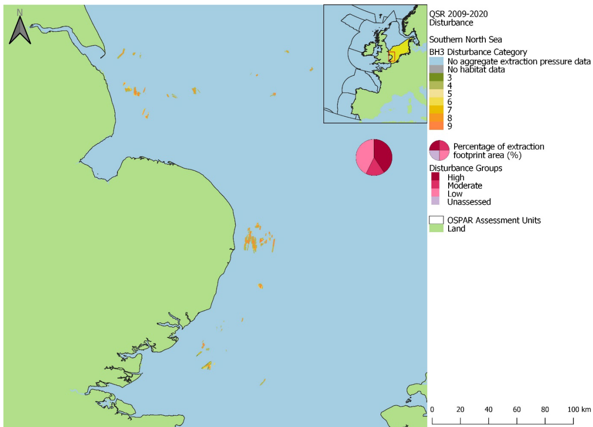
Figure bj58: Spatial distribution of extraction disturbance within the Southern North Sea assessment unit in the 2009 to 2020 assessment period. Pie charts show the percentage of the extraction footprint area under each disturbance group: 'High' (categories 8-9), 'Moderate' (categories 5-7), 'Low' (categories 1-4),
