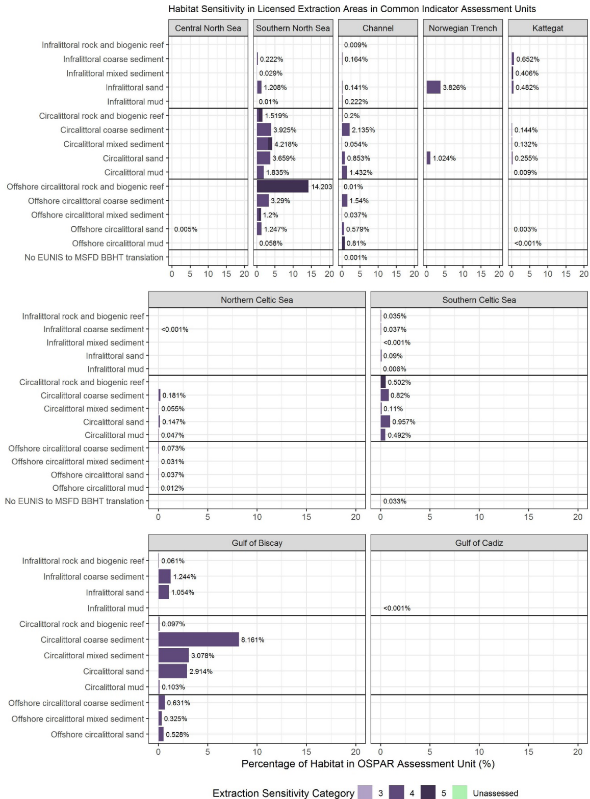
Figure o11: Percentage of Broad Habitat Type area within an assessment unit in each sensitivity category. Extraction sensitivity was only assessed within licensed areas; therefore, the numerical labels represent the total percentage of each habitat area within an assessment unit that occurred in licensed areas. No EUNIS to MSFD BBHT translation = EUNIS habitats that could not be assigned MSFD translations (e.g., lacking substrate information).
