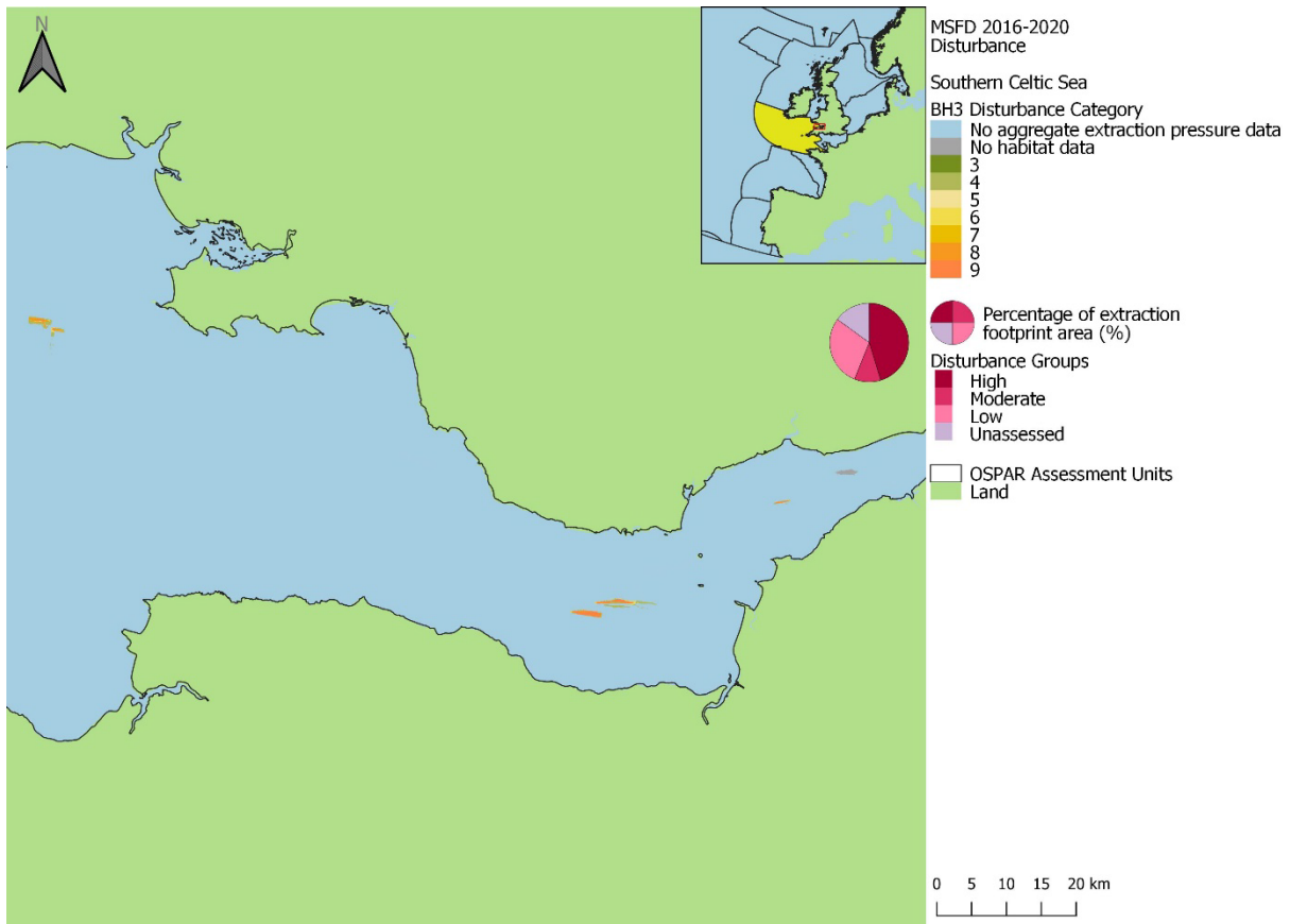
Figure bx72: Spatial distribution of extraction disturbance within the Southern Celtic Sea assessment unit in the 2016 to 2020 assessment period. Pie charts show the percentage of the extraction footprint area under each disturbance group: ‘High’ (categories 8-9), ‘Moderate’ (categories 5-7), ‘Low’ (categories 1-4), and Unassessed (area where extraction pressure was present, but disturbance could not be assessed due to i) no habitat data, or ii) no sensitivity assessments for underlying habitat).
