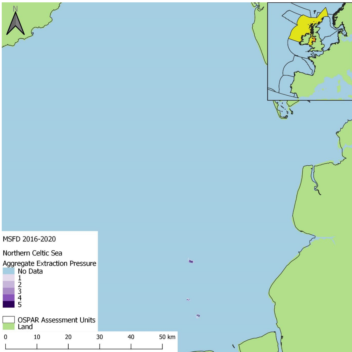
Figure aq39: Aggregated extraction pressure in the 2016 to 2020 assessment period, within the Northern Celtic Sea assessment unit.
