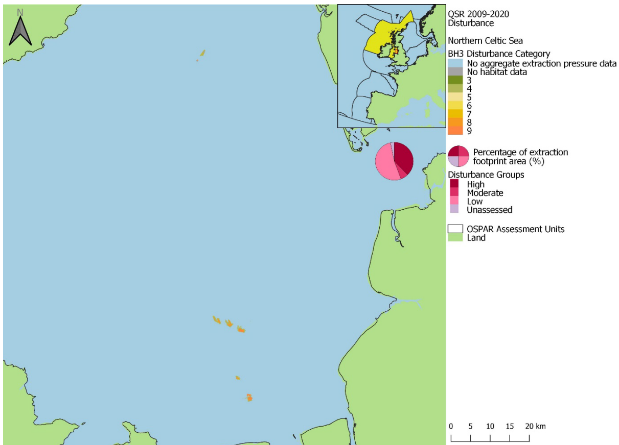
Figure bl60: Spatial distribution of extraction disturbance within the Northern Celtic Sea assessment unit in the 2009 to 2020 assessment period. Pie charts show the percentage of the extraction footprint area under each disturbance group: ‘High’ (categories 8-9), ‘Moderate’ (categories 5-7), ‘Low’ (categories 1-4), and Unassessed (area where extraction pressure was present, but disturbance could not be assessed due to i) no habitat data, or ii) no sensitivity assessments for underlying habitat).
