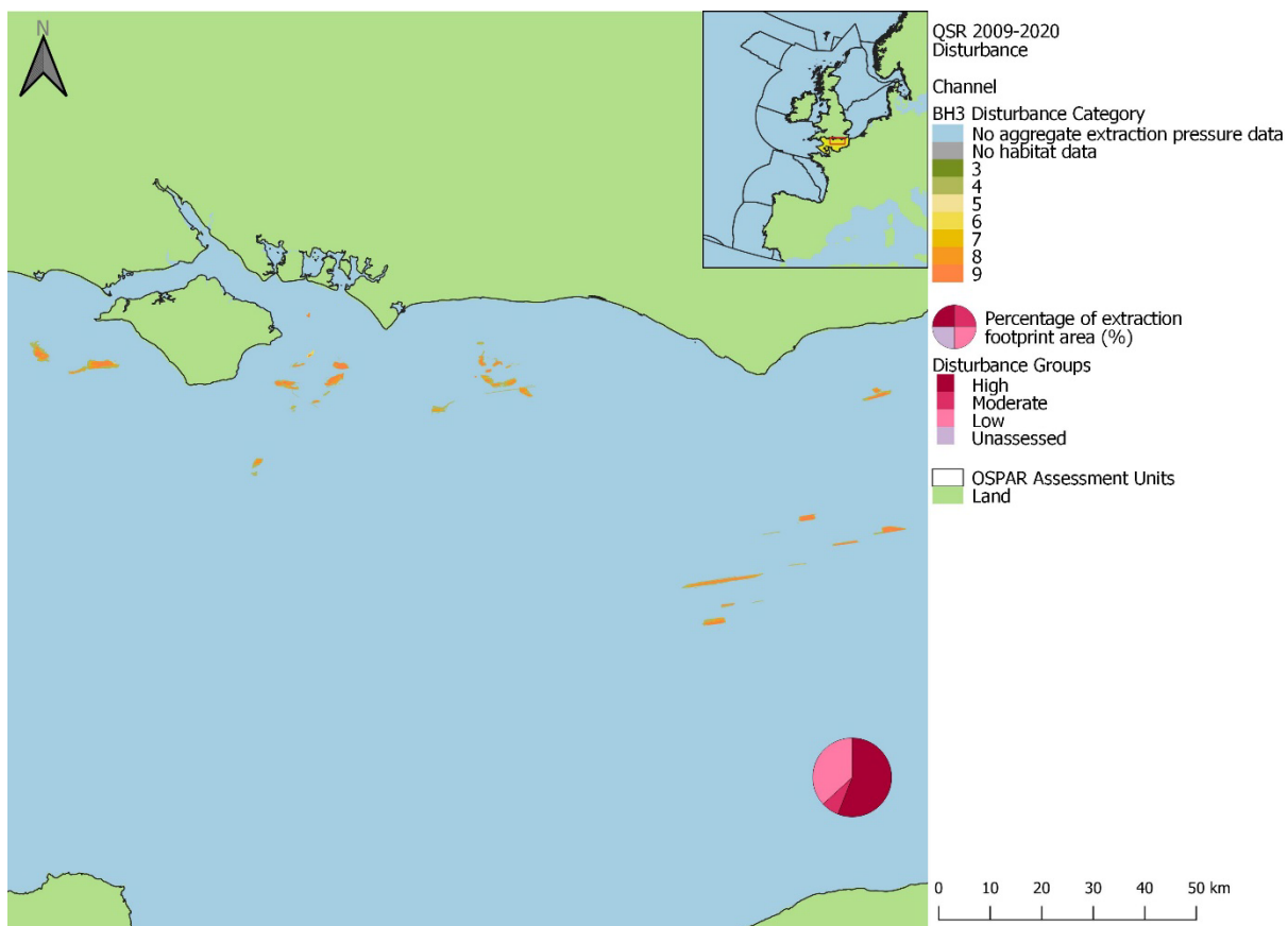
Figure bk59: Spatial distribution of extraction disturbance within the Channel assessment unit in the 2009 to 2020 assessment period. Pie charts show the percentage of the extraction footprint area under each disturbance group: ‘High’ (categories 8-9), ‘Moderate’ (categories 5-7), ‘Low’ (categories 1-4), and Unassessed (area where extraction pressure was present, but disturbance could not be assessed due to i) no habitat data, or ii) no sensitivity assessments for underlying habitat).
