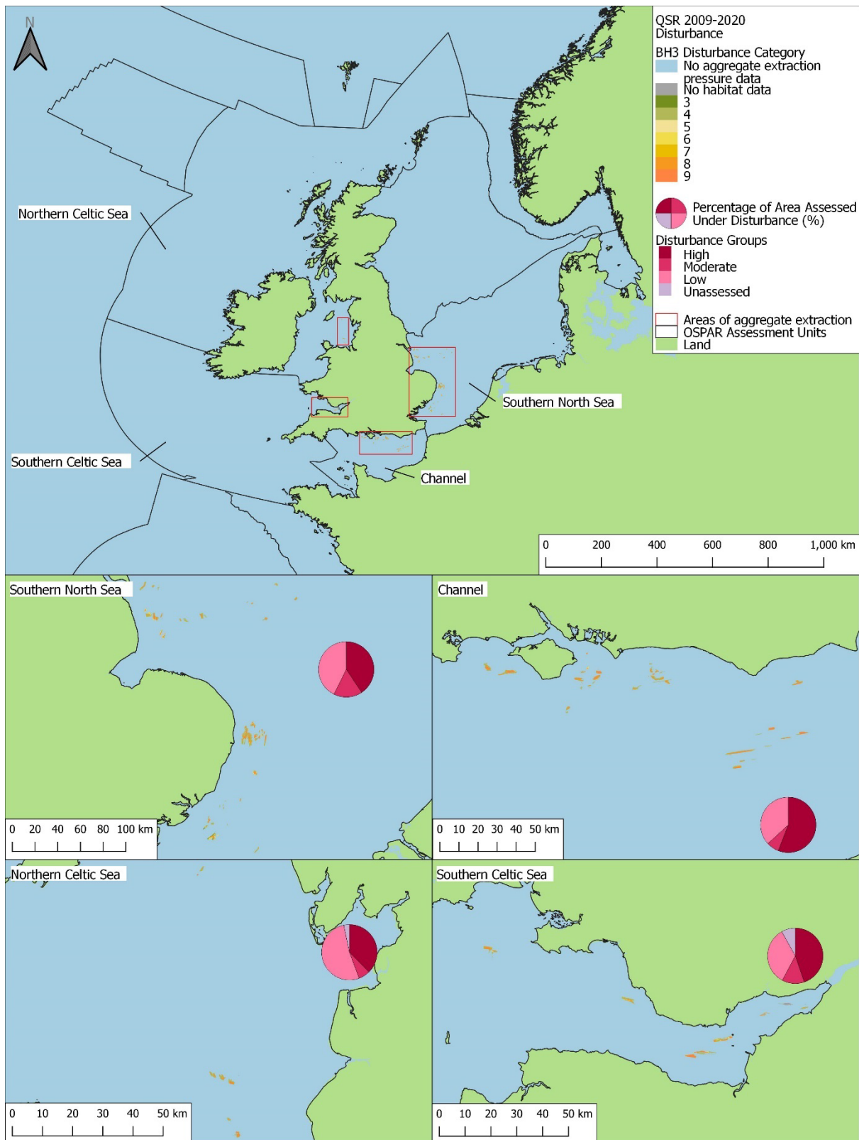
Figure 3: Spatial distribution of extraction disturbance in the 2009 to 2020 assessment period. Pie charts show the percentage of the extraction footprint area under each disturbance group: ‘High’ (categories 8-9), ‘Moderate’ (categories 5-7), ‘Low’ (categories 1-4), and Unassessed (area where extraction pressure was present, but disturbance could not be assessed due to i) no habitat data, or ii) no sensitivity assessments for underlying habitat)
