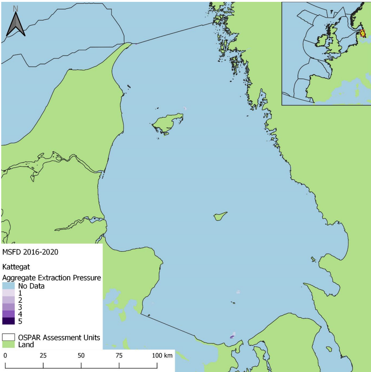
Figure ap38: Aggregated extraction pressure in the 2016 to 2020 assessment period, within the Kattegat assessment unit.
