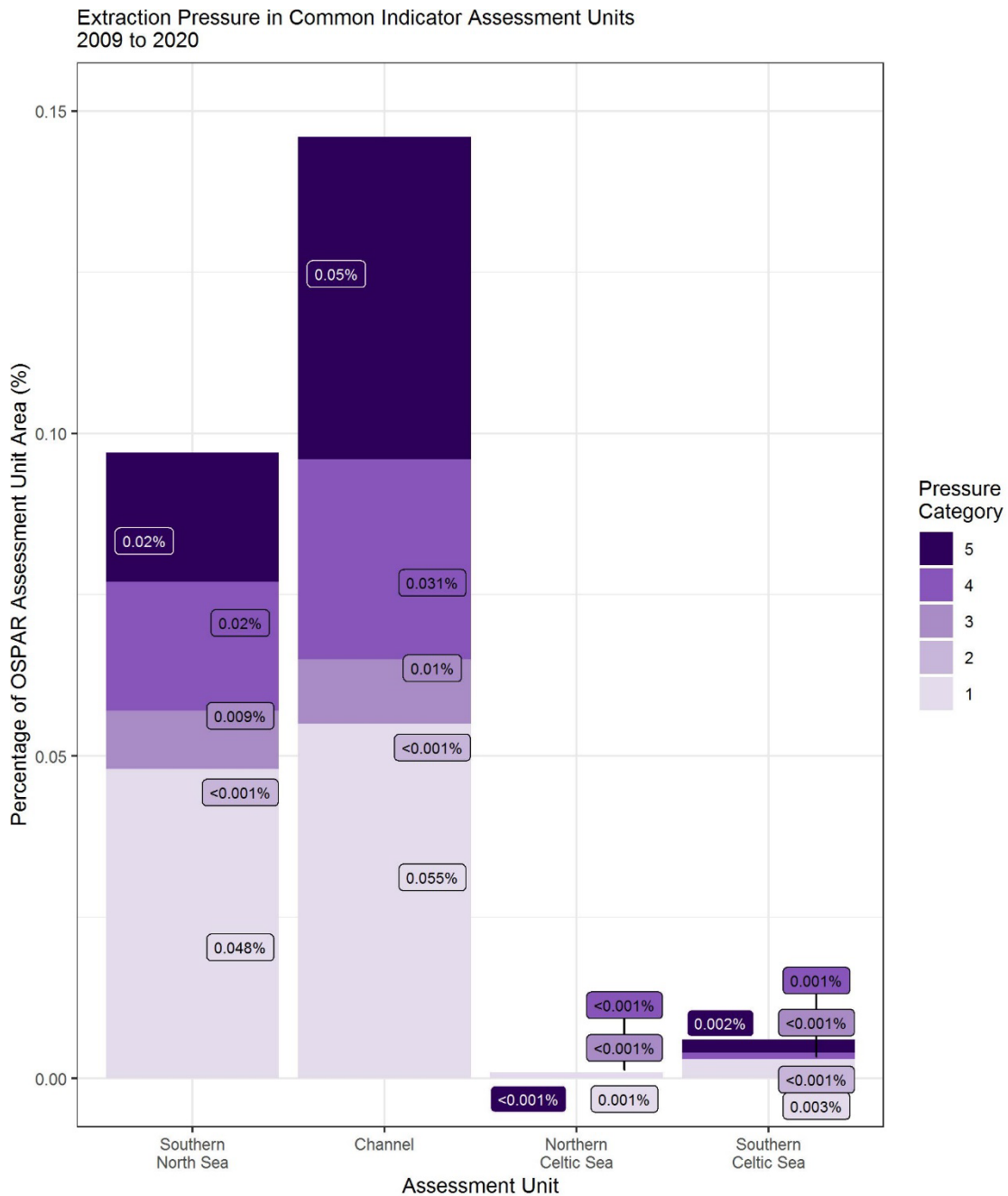
Figure ad26: Percentage of OSPAR Common Indicator Assessment Unit with extraction pressure in the 2009 to 2020 assessment period.
