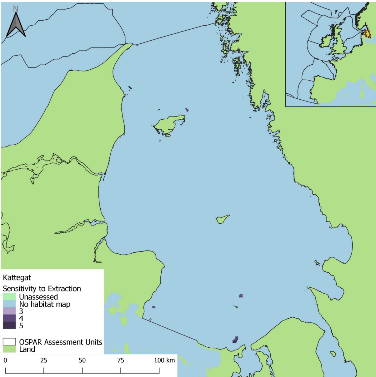
Figure s15: Extent and distribution of habitat and benthic species sensitivities (based on resilience and resistance) to extraction combined within EUNIS Level 2-6 benthic habitat types, where aggregate extraction pressure data were available in the Kattegat assessment unit.
