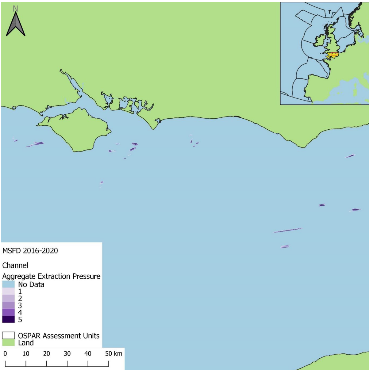
Figure an36: Aggregated extraction pressure in the 2016 to 2020 assessment period, within the Channel assessment unit.
