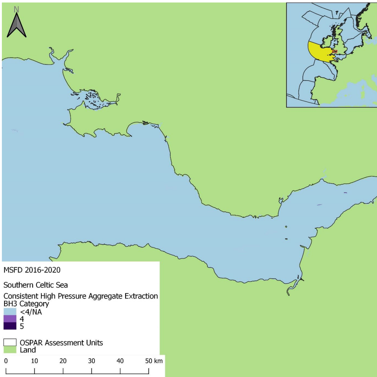
Figure bh56: Spatial distribution of consistently high (category 4 or 5) extraction pressure within the 2016 to 2020 assessment period in the Southern Celtic Sea assessment period. Grid cells were considered to have ‘Consistent’ pressure if a change in less than three pressure categories was observed within the assessment period.
