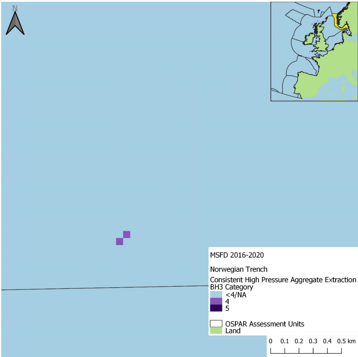
Figure be53: Spatial distribution of consistently high (category 4 or 5) extraction pressure within the 2016 to 2020 assessment period in the Norwegian Trench assessment period. Grid cells were considered to have 'Consistent' pressure if a change in less than three pressure categories was observed within the assessment period.
