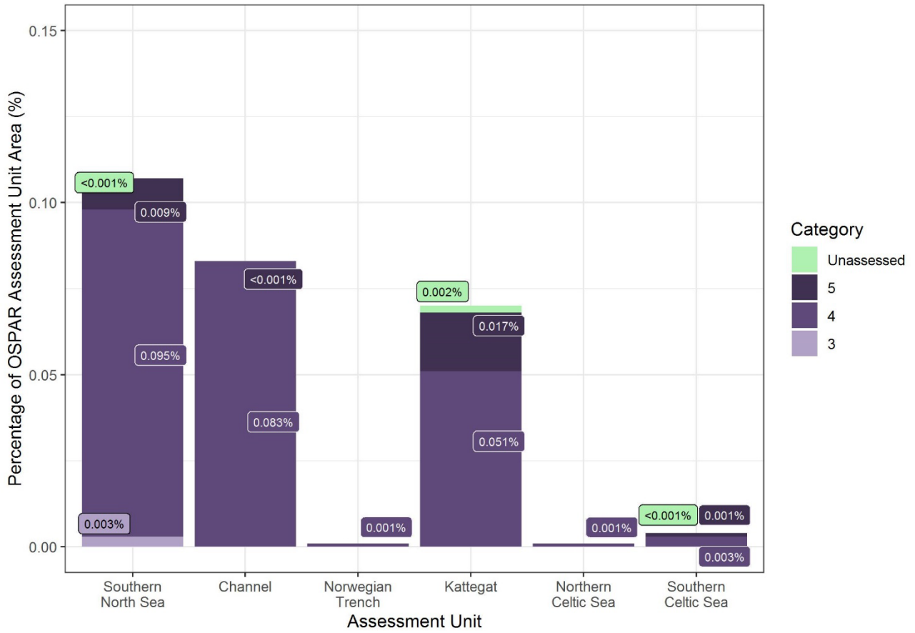
Figure x20: Percentage of OSPAR Common Indicator Assessment Unit with extraction pressure in the 2016 to 2020 assessment period for each extraction sensitivity category.
