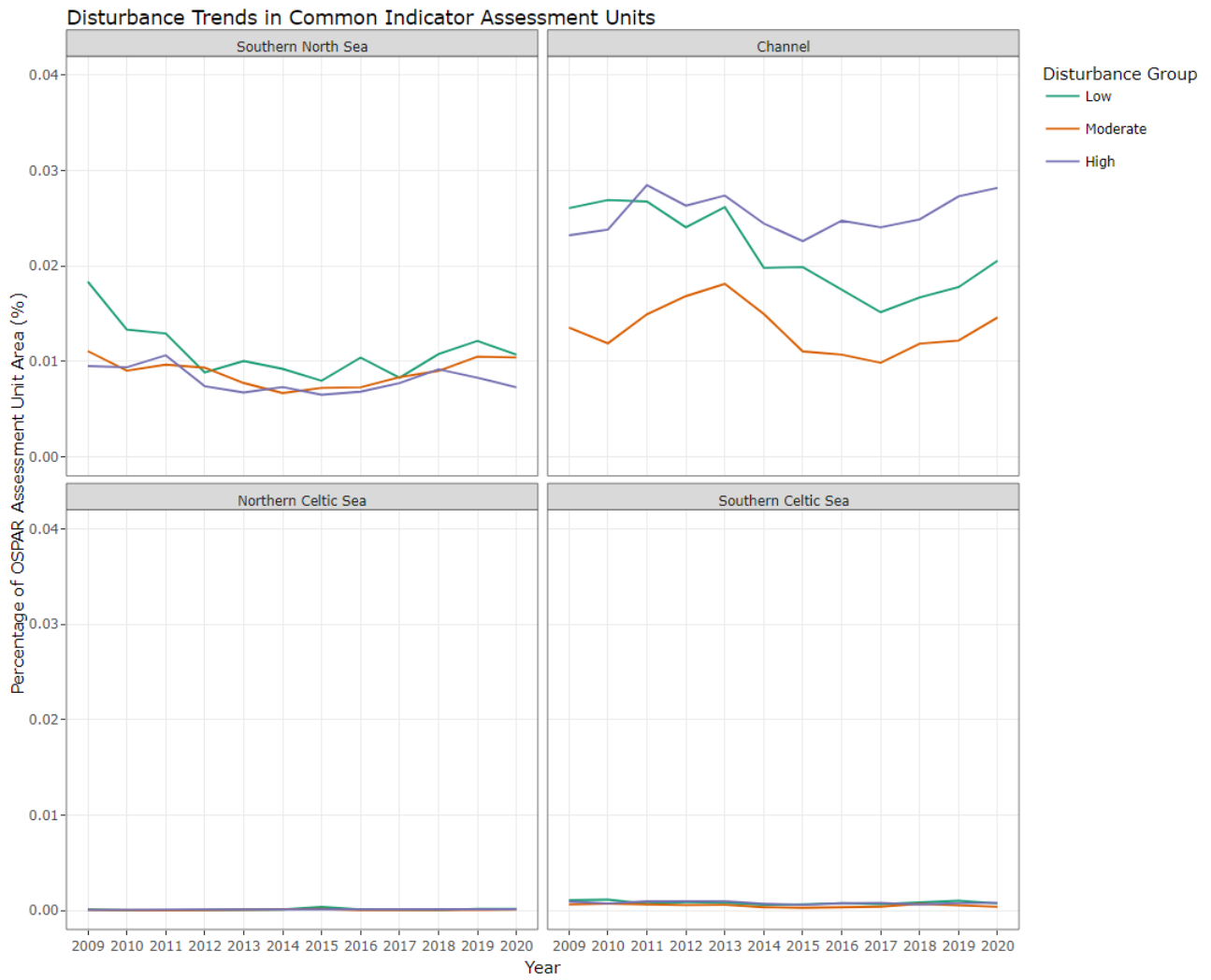
Figure bp64: The annual percentage of OSPAR benthic assessment unit areas (where BH3 is agreed as an OSPAR Common Indicator) under the disturbance groups ‘Low’ (disturbance categories 1-4), ‘Moderate’ (disturbance categories 5-7) and ‘High’ (disturbance categories 8 and 9) between the years 2009 to 2020. Note, only data covering the entire assessment period is shown (United Kingdom).
