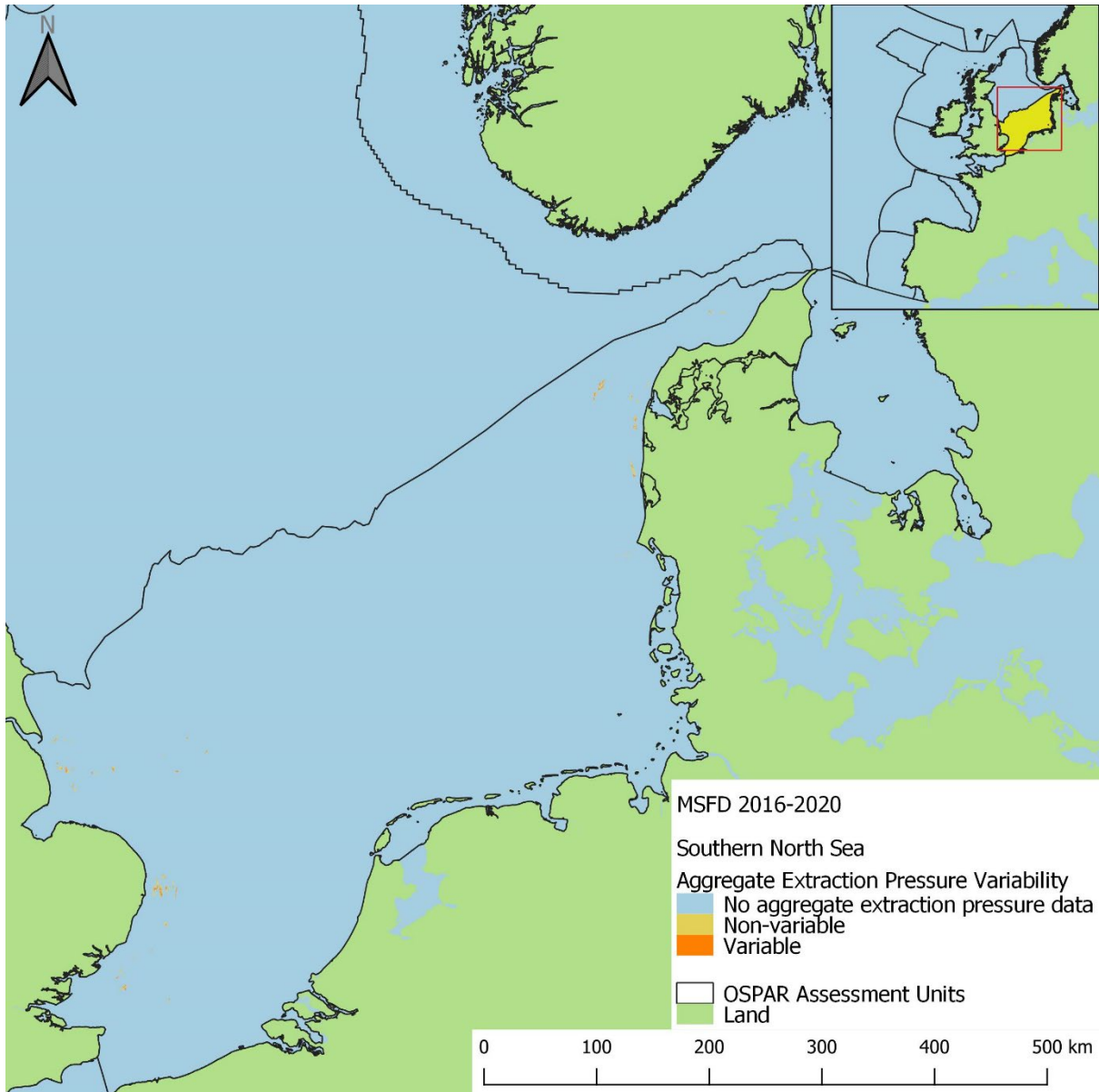
Figure av44: Spatial distribution of ‘Variable’ and ‘Non-variable’ extraction pressure in the 2016 to 2020 assessment period in the Southern North Sea assessment unit. Grid cells were categorised ‘Variable’ if a range of three or more pressure categories was observed throughout the time series.
