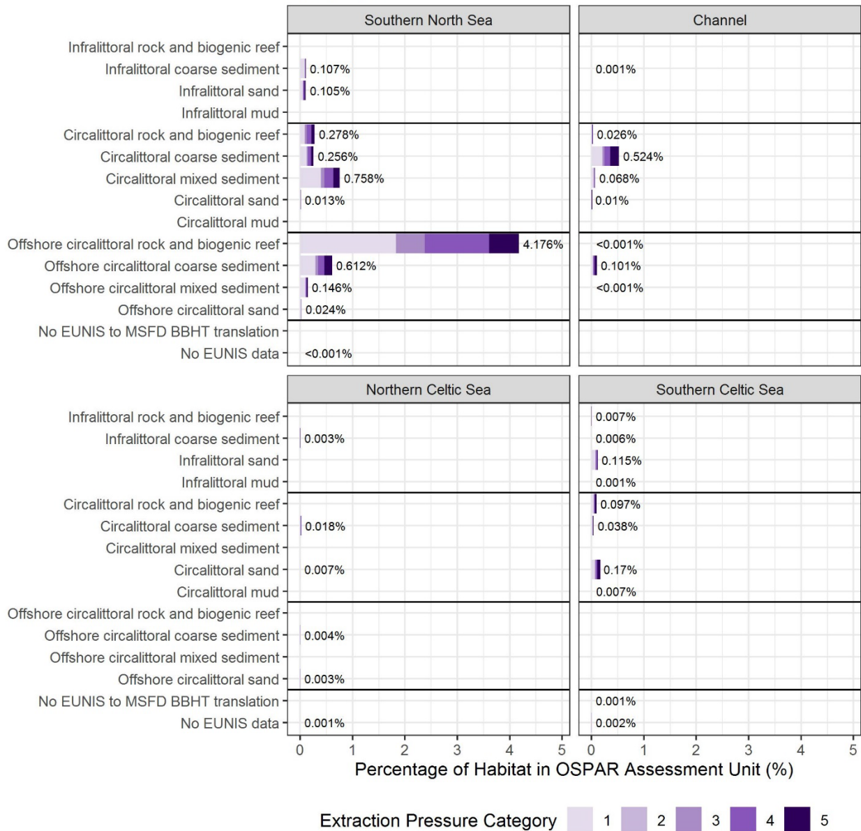
Figure af28: The percentage of Broad Habitat Types in OSPAR Common Indicator Assessment Units with extraction pressure in the 2009 to 2020 assessment period.
