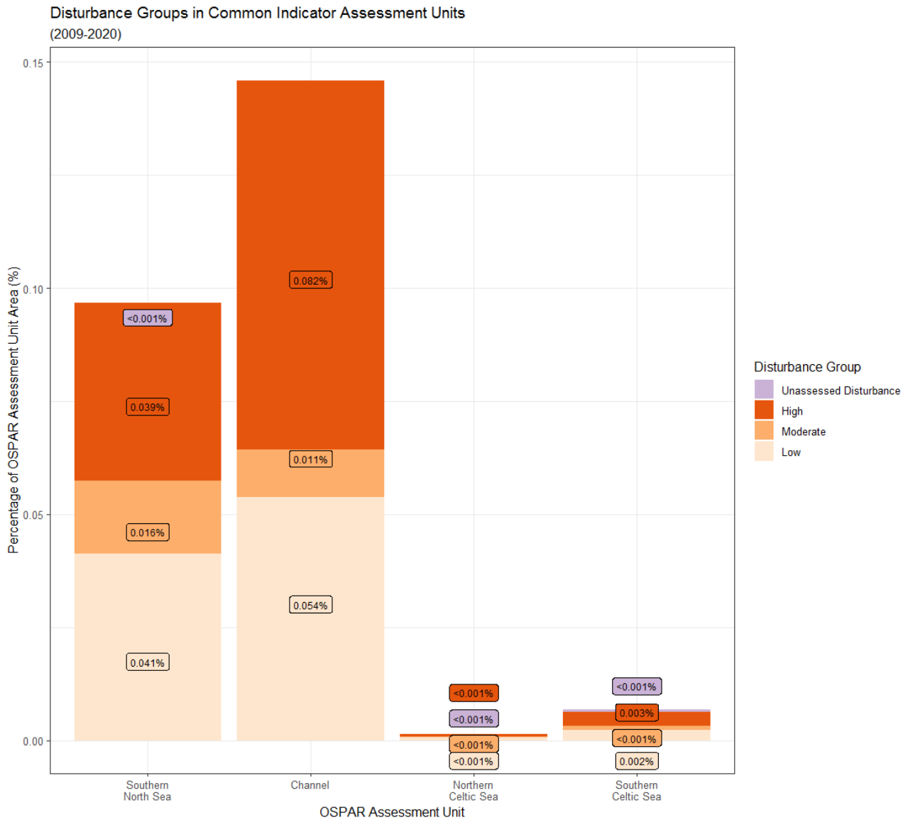
Figure bn62: The percentage of OSPAR Common Indicator Assessment Units under each of the following disturbance groups in the 2009 to 2020 assessment period: ‘Unassessed Disturbance’ = area where extraction pressure was present but disturbance could not be assessed due to i) no habitat data, or ii) no sensitivity assessments for underlying habitat; ‘Low’ = disturbance categories 1-4; ‘Moderate’ = disturbance categories 5-7; ‘High’ = disturbance categories 8 and 9. Horizontal black lines represent the separation in biological zones.
