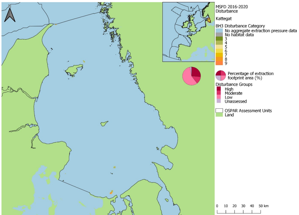
Figure bv70: Spatial distribution of extraction disturbance within the Kattegat assessment unit in the 2016 to 2020 assessment period. Pie charts show the percentage of the extraction footprint area under each disturbance group: ‘High’ (categories 8-9), ‘Moderate’ (categories 5-7), ‘Low’ (categories 1-4), and Unassessed (area where extraction pressure was present, but disturbance could not be assessed due to i) no habitat data, or ii) no sensitivity assessments for underlying habitat).
