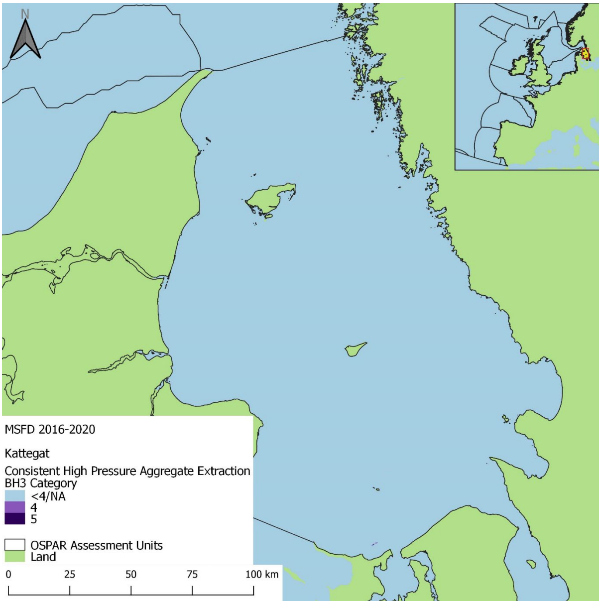
Figure bf54: Spatial distribution of consistently high (category 4 or 5) extraction pressure within the 2016 to 2020 assessment period in the Kattegat assessment period. Grid cells were considered to have ‘Consistent’ pressure if a change in less than three pressure categories was observed within the assessment period.
