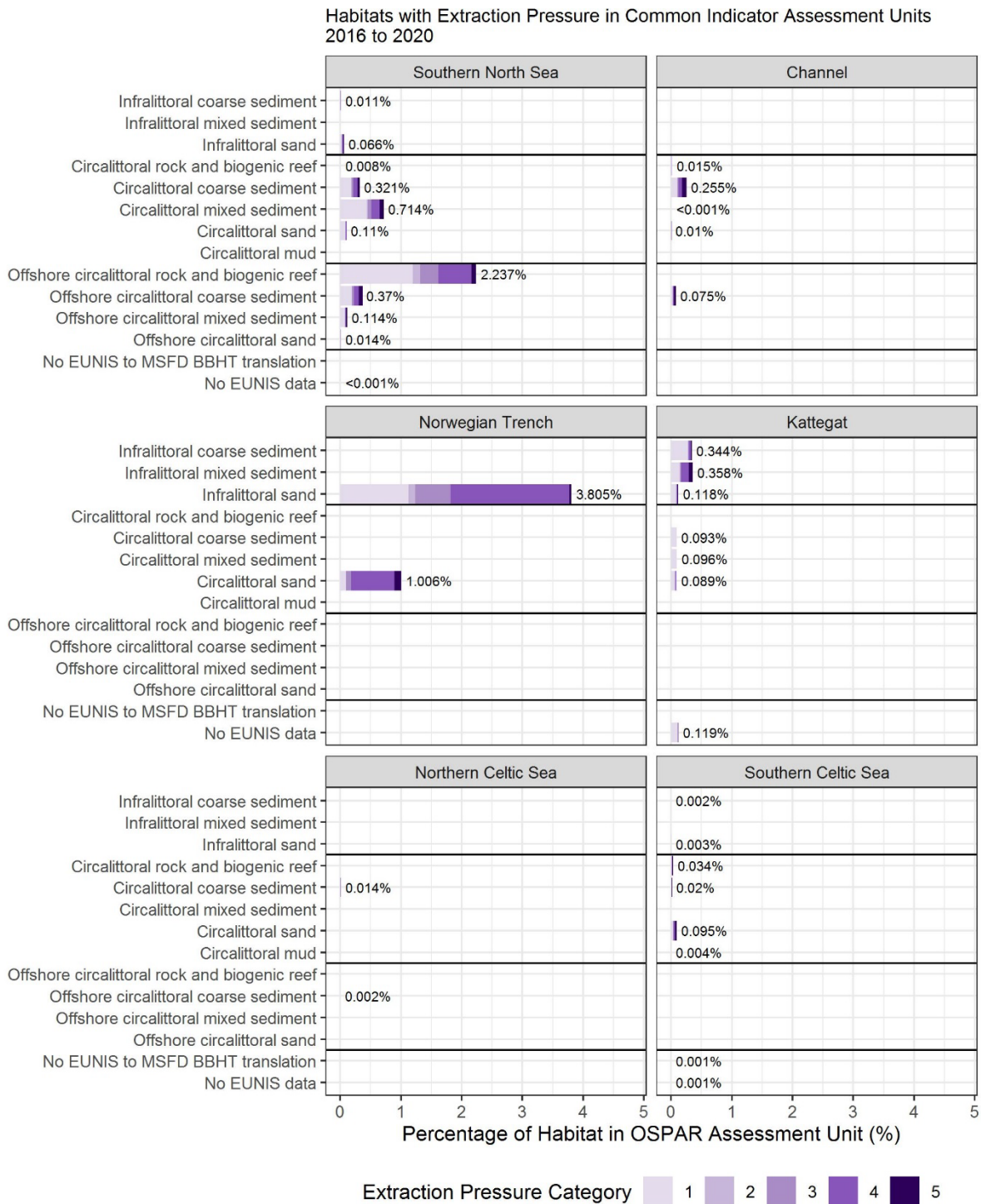
Figure au43: The percentage of Broad Benthic Habitat Types in OSPAR Common Indicator Assessment Units with extraction pressure in the 2016 to 2020 assessment period. No EUNIS to MSFD BBHT translation = EUNIS habitats that couldn't be assigned MSFD translations (e.g., lacking substrate information).
