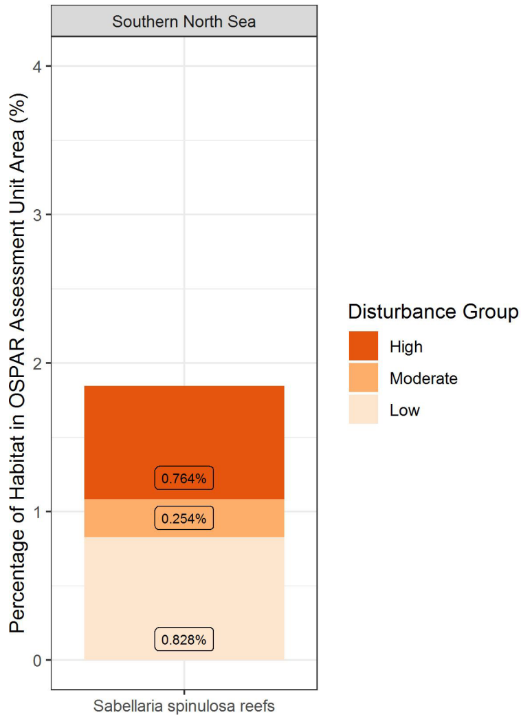
Figure cb76: The percentage of OSPAR Threatened and / or Declining Habitats in each OSPAR Common Indicator Assessment Unit under each of the following disturbance groups in the 2009 to 2020 assessment period: ‘Low’ = disturbance categories 1-4; ‘Moderate’ = disturbance categories 5-7; ‘High’ = disturbance categories 8 and 9.
