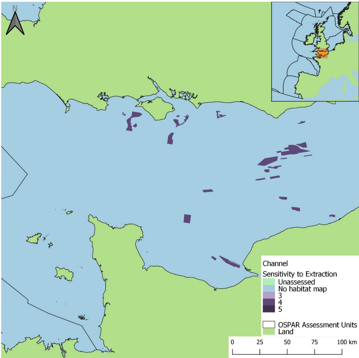
Figure g3: Sensitivity map of areas licensed for extraction in the Channel.
