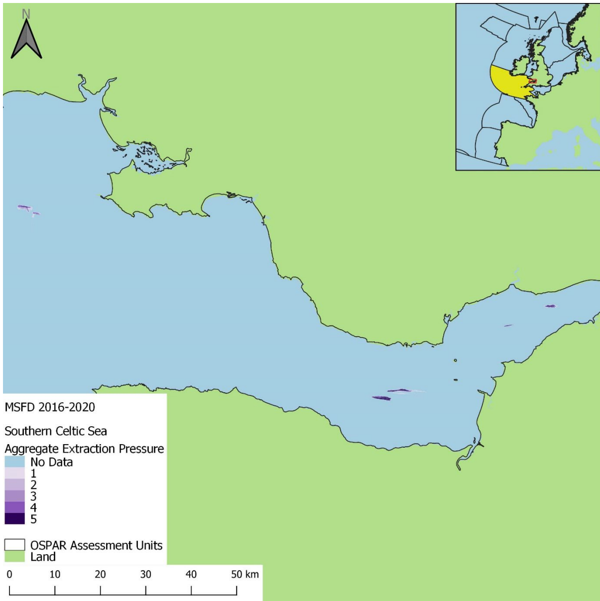
Figure ar40: Aggregated extraction pressure in the 2016 to 2020 assessment period, within the Southern Celtic Sea assessment unit.
