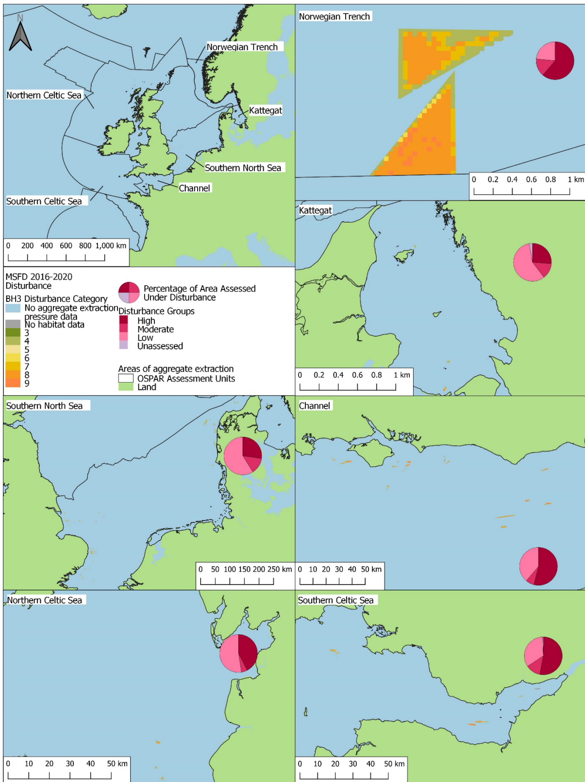
Figure 4: Spatial distribution of extraction disturbance in the 2016 to 2020 assessment period. Pie charts show the percentage of the extraction footprint area under each disturbance group: ‘High’ (categories 8-9), ‘Moderate’ (categories 5-7), ‘Low’ (categories 1-4), and Unassessed (area where extraction pressure was present, but disturbance could not be assessed due to i) no habitat data, or ii) no sensitivity assessments for underlying habitat)
