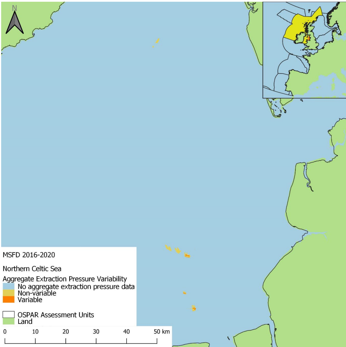
Figure az48: Spatial distribution of 'Variable' and 'Non-variable' extraction pressure in the 2016 to 2020 assessment period in the Northern Celtic Sea assessment unit. Grid cells were categorised 'Variable' if a range of three or more pressure categories was observed throughout the time series.
