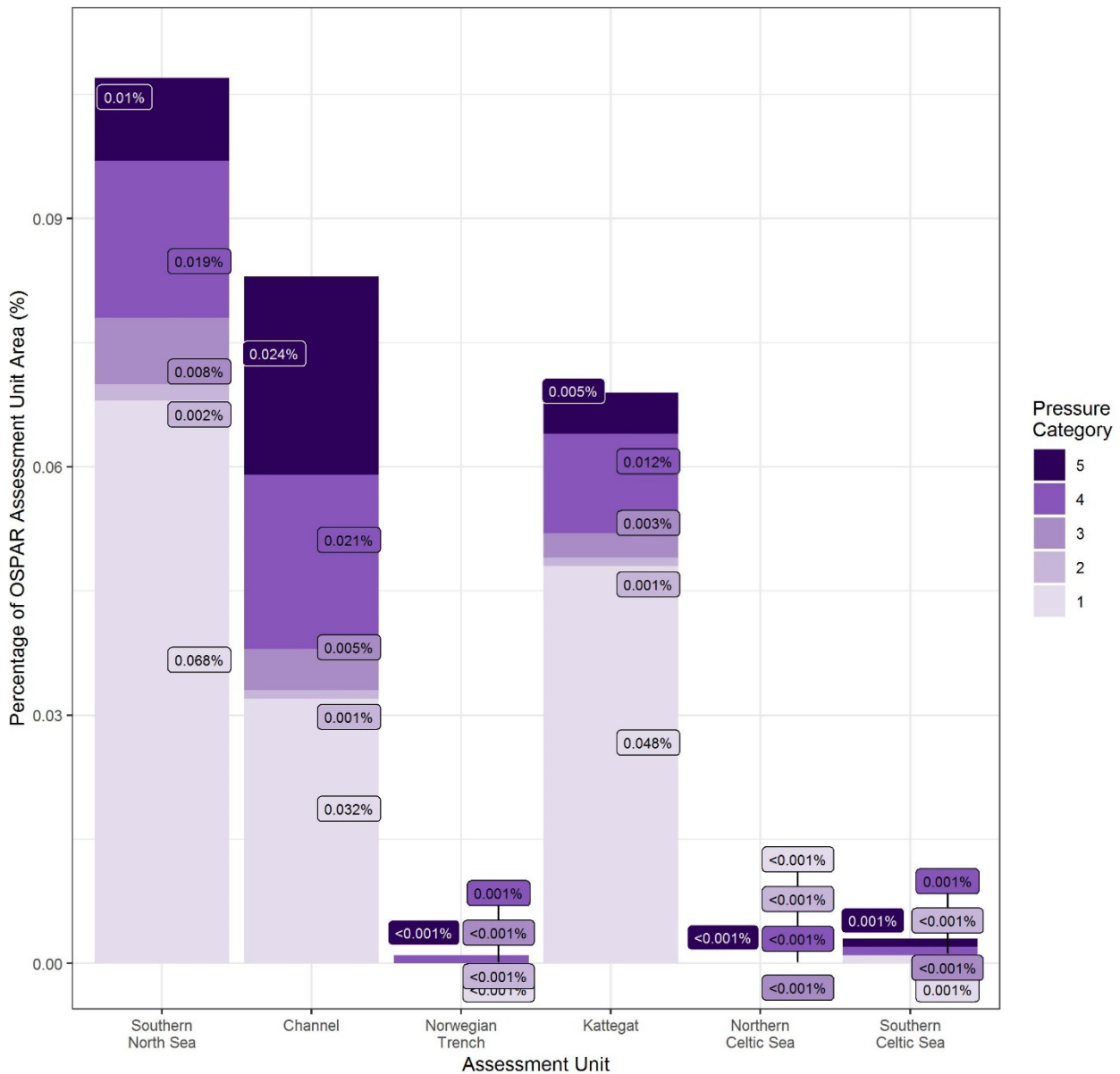
Figure as41: Percentage of OSPAR Common Indicator Assessment Unit with extraction pressure in the 2016 to 2020 assessment period.
