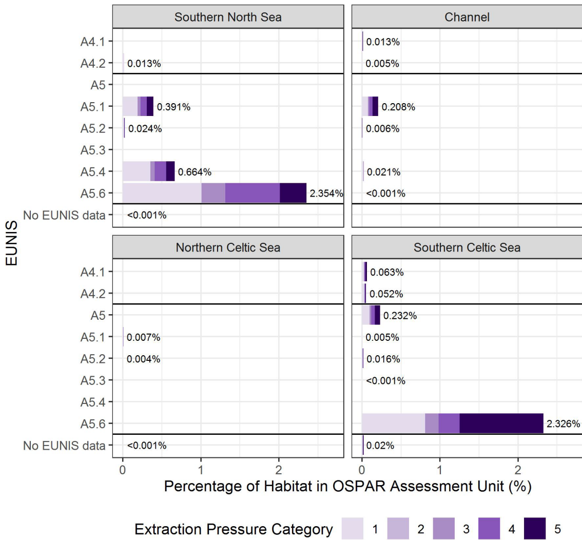
Habitats with Extraction Pressure in Common Indicator Assessment Units 2009 to 2020
