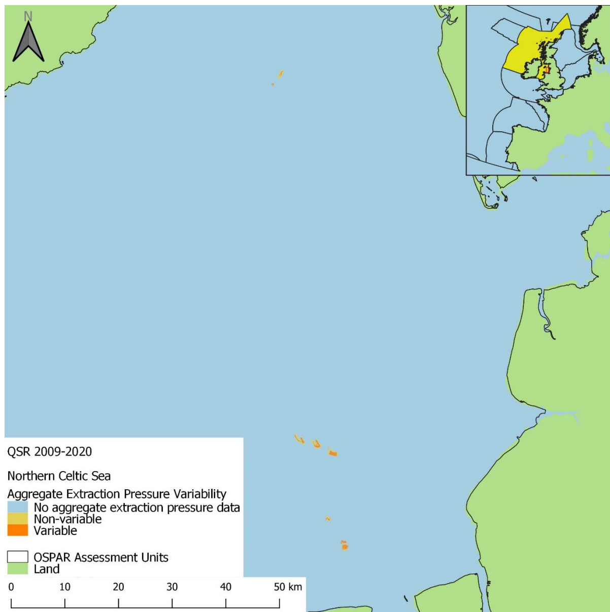
Figure ai31: Spatial distribution of 'Variable' and 'Non-variable' extraction pressure in the 2009 to 2020 assessment period in the Northern Celtic Sea assessment unit. Grid cells were categorised 'Variable' if a range of three or more pressure categories was observed throughout the time series.
