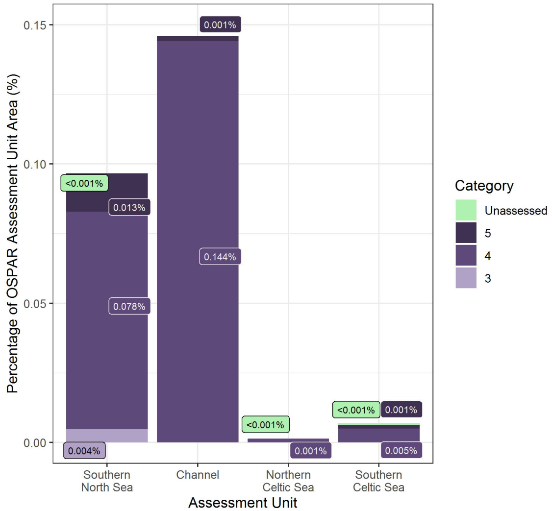
Figure v18: Percentage of OSPAR Common Indicator Assessment Unit with extraction pressure in the 2009 to 2020 assessment period for each extraction sensitivity category.
