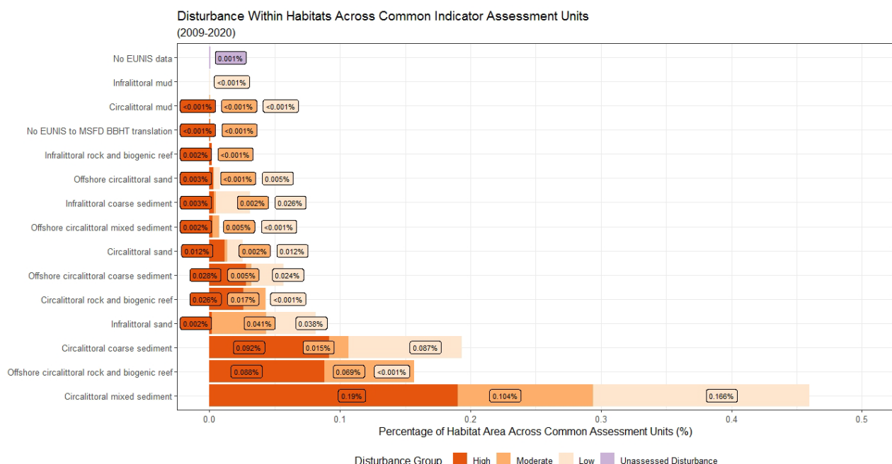
Figure bi57: The percentage of each distinct Broad Habitat Type’s area across OSPAR benthic assessment units that contained extraction intensity data from the United Kingdom (Southern North Sea, Channel, Northern Celtic Sea, Southern Celtic Sea) under each of the following disturbance groups in the 2009 to 2020 assessment period: ‘High’ = disturbance categories 8 and 9; ‘Moderate’ = disturbance categories 5-
