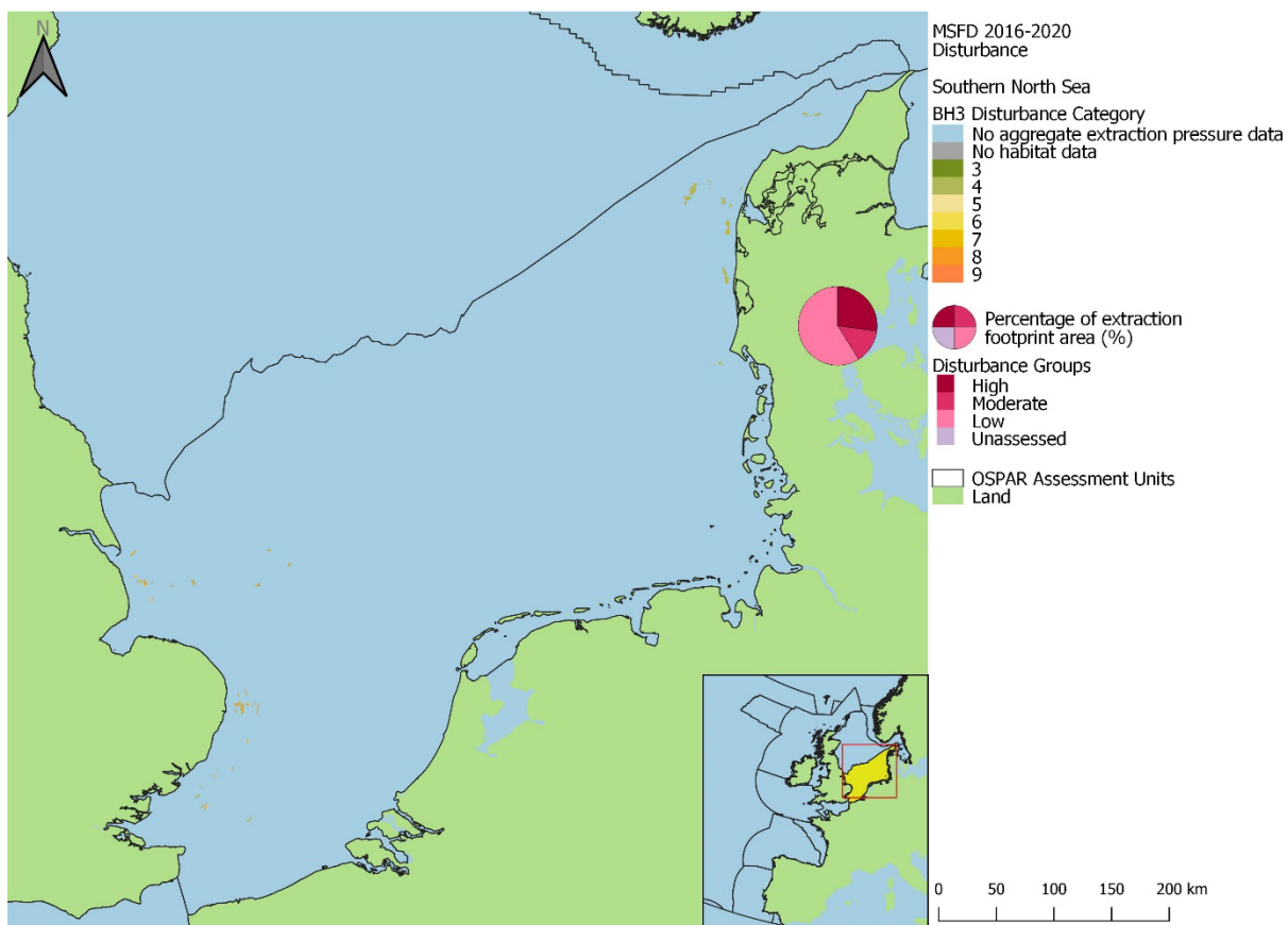
Figure bs67: Spatial distribution of extraction disturbance within the Southern North Sea assessment unit
