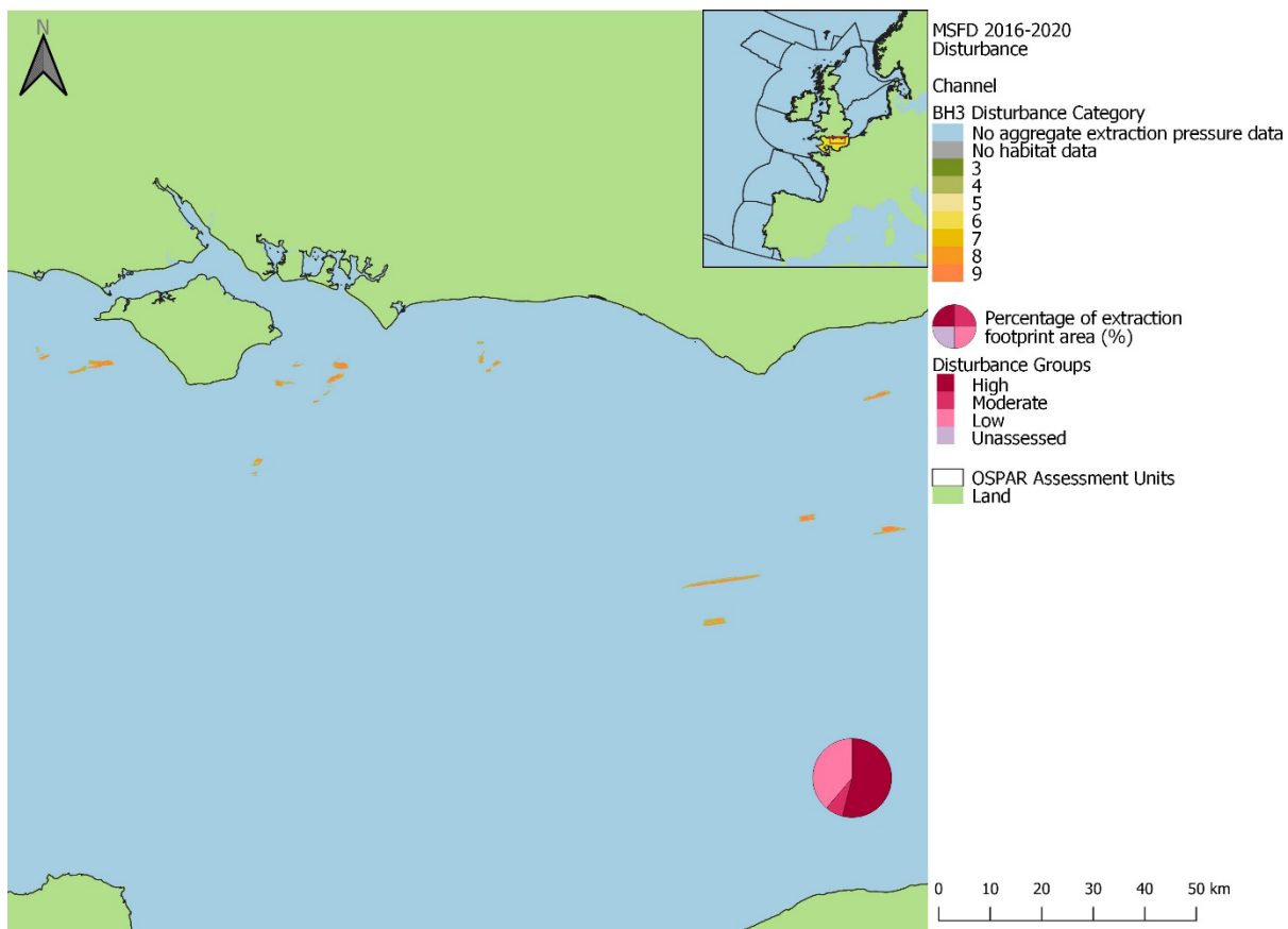
Figure bt68: Spatial distribution of extraction disturbance within the Channel assessment unit in the 2016 to 2020 assessment period. Pie charts show the percentage of the extraction footprint area under each disturbance group: ‘High’ (categories 8-9), ‘Moderate’ (categories 5-7), ‘Low’ (categories 1-4), and Unassessed (area where extraction pressure was present, but disturbance could not be assessed due to i) no habitat data, or ii) no sensitivity assessments for underlying habitat).
