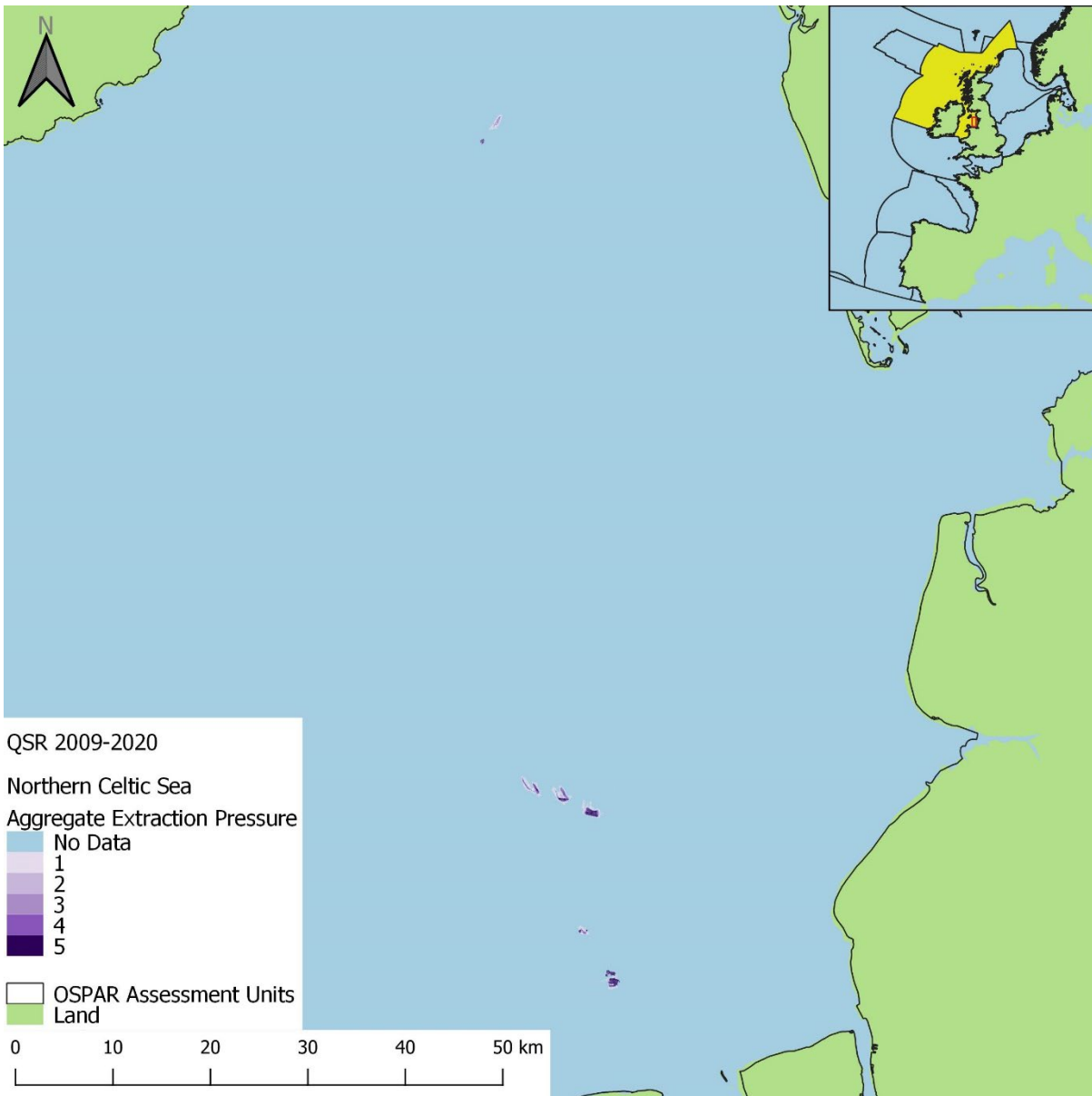
Figure ab24: Aggregated extraction pressure in the 2009 to 2020 assessment period, within the Northern Celtic Sea assessment unit.
