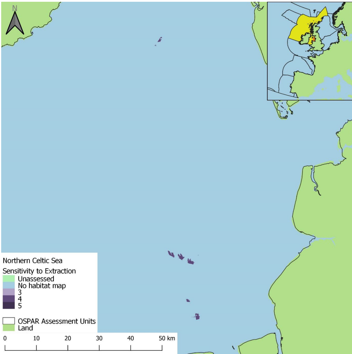
Figure t16: Extent and distribution of habitat and benthic species sensitivities (based on resilience and resistance) to extraction combined within EUNIS Level 2-6 benthic habitat types, where aggregate extraction pressure data were available in the Northern Celtic Sea assessment unit.
