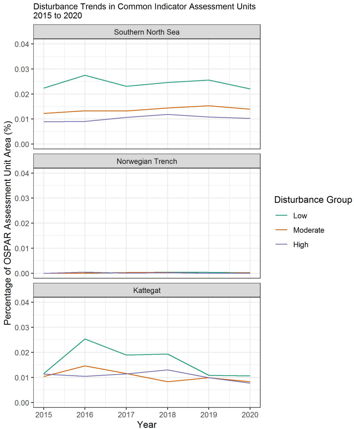
Figure bq65: The annual percentage of OSPAR benthic assessment unit areas (where BH3 is agreed as an OSPAR Common Indicator) under the disturbance groups ‘Low’ (disturbance categories 1-4), ‘Moderate’ (disturbance categories 5-7) and ‘High’ (disturbance categories 8 and 9) between the years 2015 to 2020. Note, the Southern North Sea includes data from the United Kingdom and Denmark.
