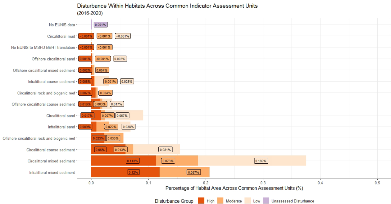
Figure br66: The percentage of each distinct Broad Habitat Type’s area across OSPAR benthic assessment units where extraction intensity data was present for the United Kingdom and Denmark (Southern North Sea, Channel, Norwegian Trench, Kattegat, Northern Celtic Sea, Southern Celtic Sea) under each of the following disturbance groups in the 2016 to 2020 assessment period: ‘High’ = disturbance categories 8 and 9; ‘Moderate’ = disturbance categories 5-7; ‘Low’ = disturbance categories 1-4; ‘Unassessed
