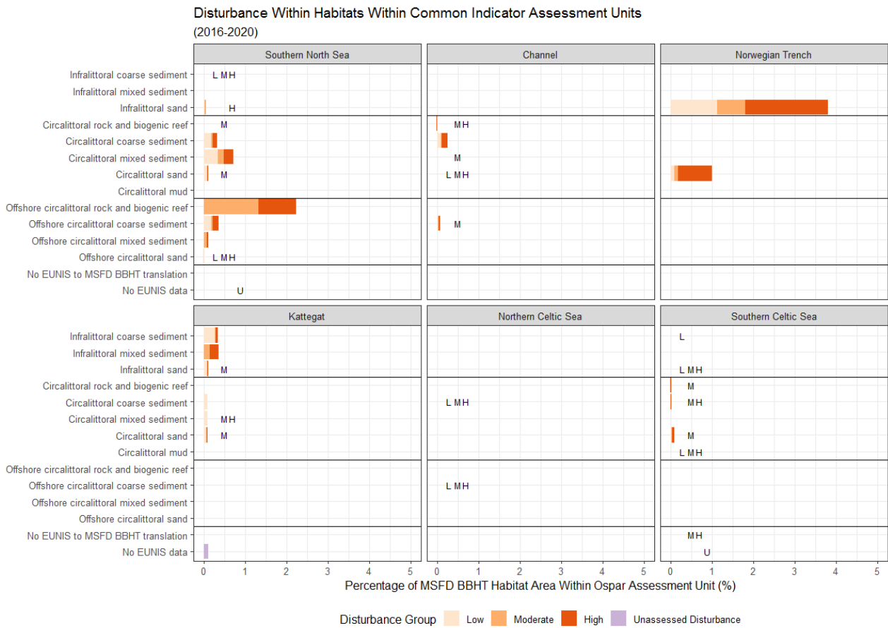
Figure bz74: The percentage of Broad Habitat Type in each OSPAR Common Indicator Assessment Units under each of the following disturbance groups in the 2016 to 2020 assessment period: ‘Unassessed Disturbance’ = area where extraction pressure was present but disturbance could not be assessed due to i) no habitat data, or ii) no sensitivity assessments for underlying habitat; ‘Low’ = disturbance categories 1-4; ‘Moderate’ = disturbance categories 5-7; ‘High’ = disturbance categories 8 and 9. Horizontal black lines represent the separation in biological zones. Disturbance groups that were present but covered <= 0,01% of a habitat area are represented by text labels where L = ‘Low’, M = ‘Moderate’, H = ‘High’, and U = ‘Unassessed Disturbance’.
