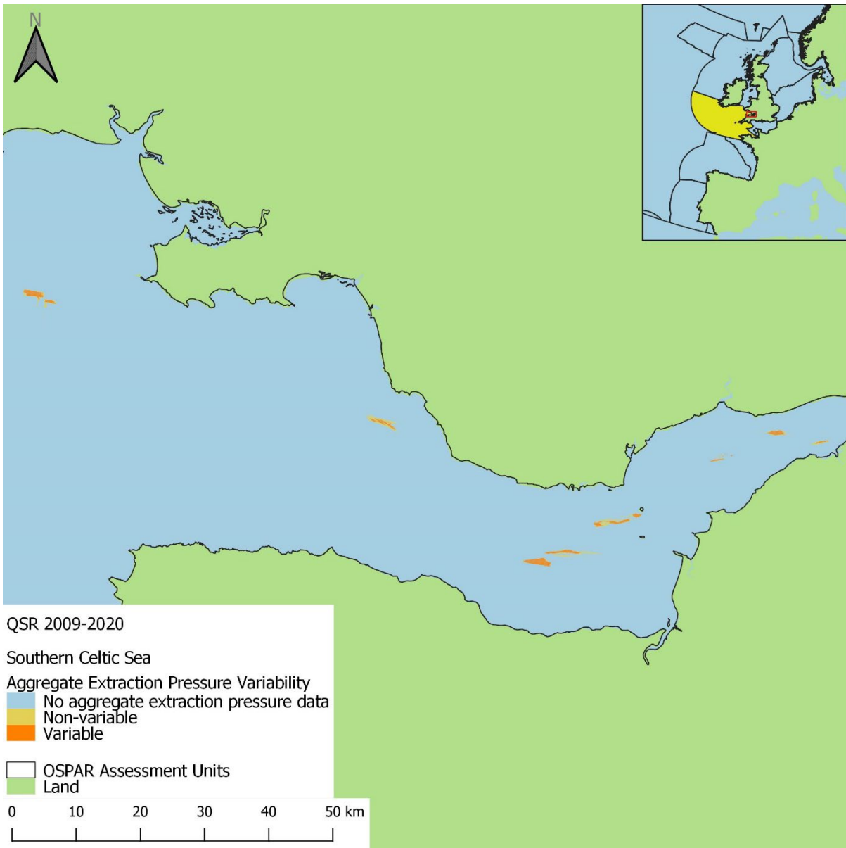
Figure aj32: Spatial distribution of 'Variable' and 'Non-variable' extraction pressure in the 2009 to 2020 assessment period in the Southern Celtic Sea assessment unit. Grid cells were categorised 'Variable' if a range of three or more pressure categories was observed throughout the time series.
